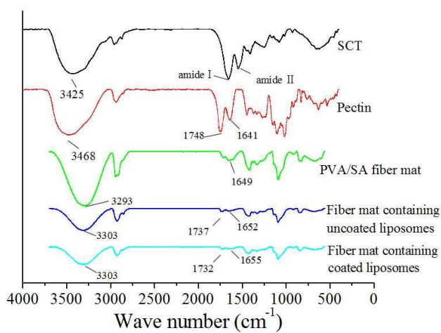
FigS.1. FTIR spectra of different samples
