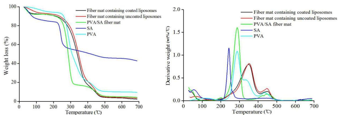
FigS.2. TG and DTG curves of different samples.
