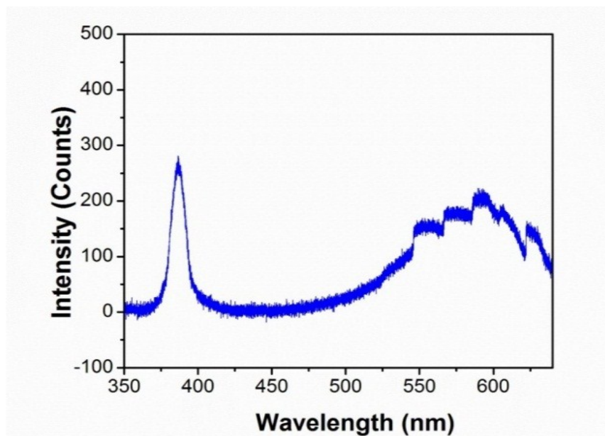
Figure S1 Room-temperature photoluminescence spectrum of as-grown ZnO nanowires.
