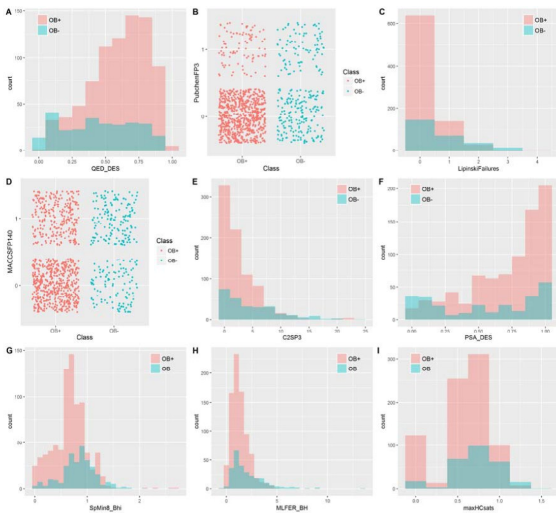
Figure S3 Distributions of top-9 molecular properties for OB data
