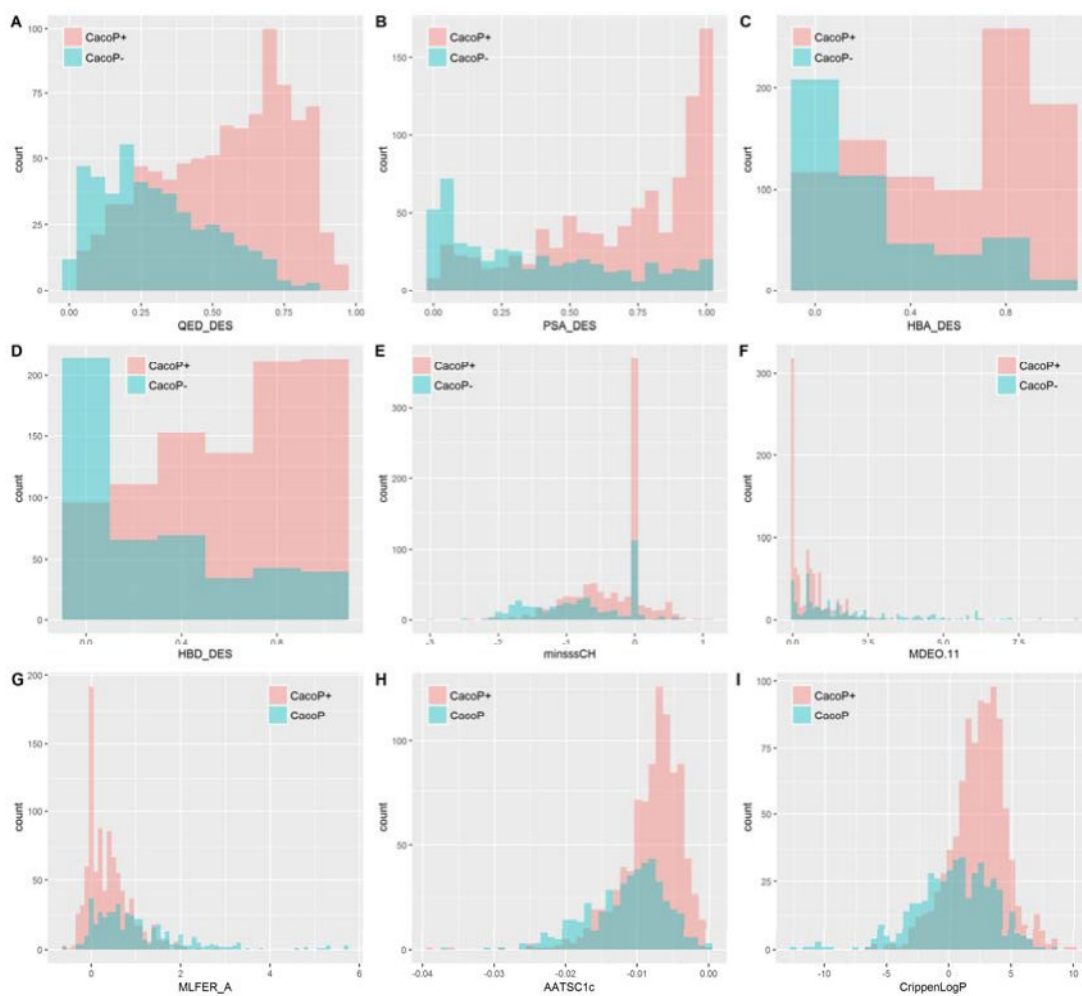
Figure S1 Distributions of top-9 molecular properties for CacoP data
