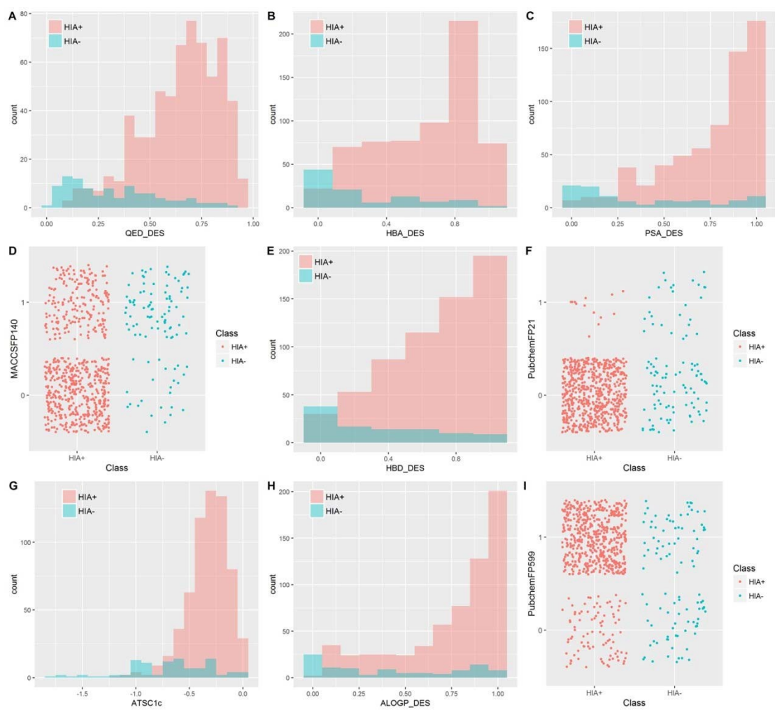
Figure S2 Distributions of top-9 molecular properties for HIA data
