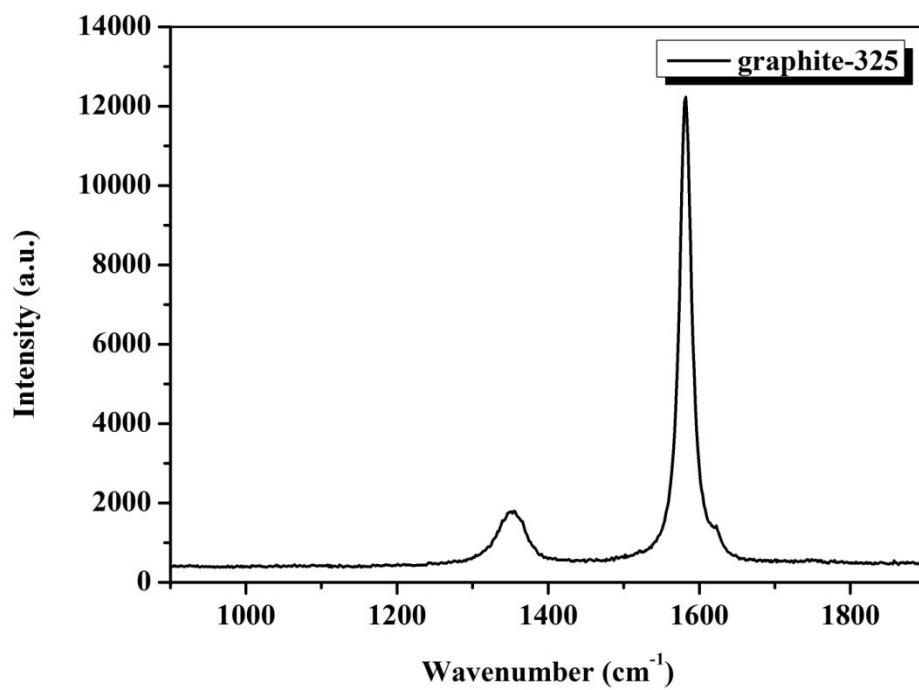
Fig. S1 Raman spectrum of graphite-325
