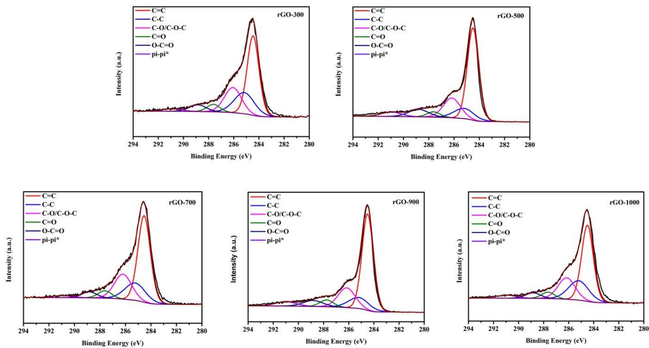
Fig. S2 C1s spectra of (a)rGO-300, (b)rGO-500, (c)rGO-700, (d)rGO-900 and (e)rGO-1000.
