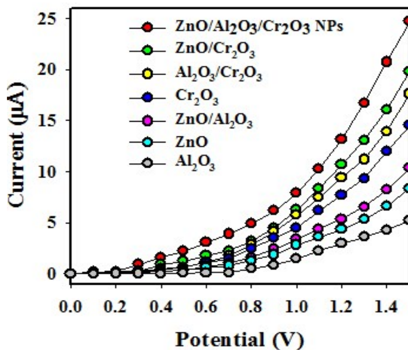
Fig. S1: Control experiment is performed based on different composition of fabricated GCE such as Al 2 O 3 , ZnO, Cr 2 O 3 , ZnO/Al 2 O 3 , Al 2 O 3 /Cr 2 O 3 , ZnO/Cr 2 O 3 and ZnO/Al 2 O 3 /Cr 2 O 3 nanoparticles.
