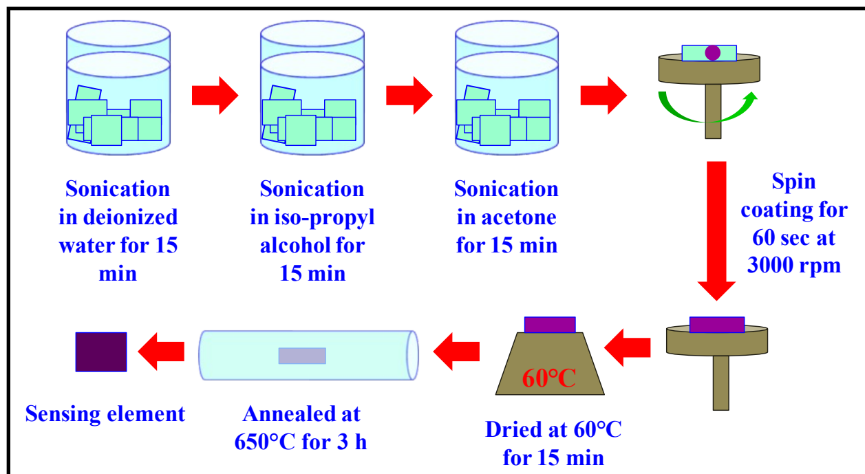
Fig. Schematic for fabrication of sensing element
