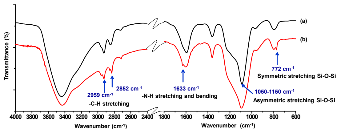
Figure S2 FTIR spectra of (a) MS and (b) MS-NH 2 nanoparticles.
