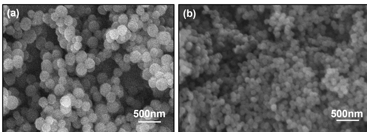
Figure S1 Scanning electron micrographs of (a) SiO 2 (b) MS- SiO 2 .
