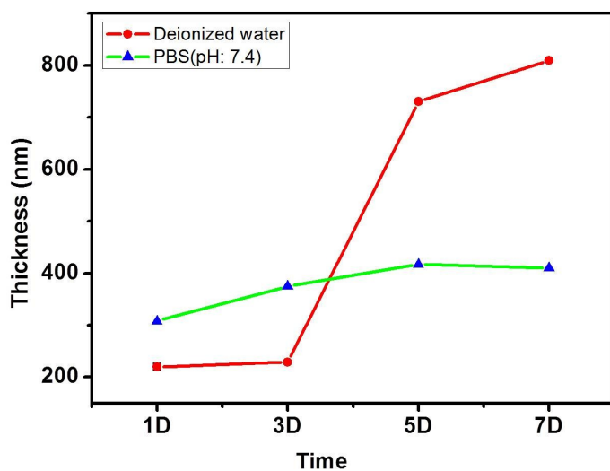
Fig. S2. Thickness of Ti-PDA-M(P) was immersed in deionized water and PBS(pH: 7.4) for 1, 3, 5 and 7 days (1D, 3D, 5D and 7D).
