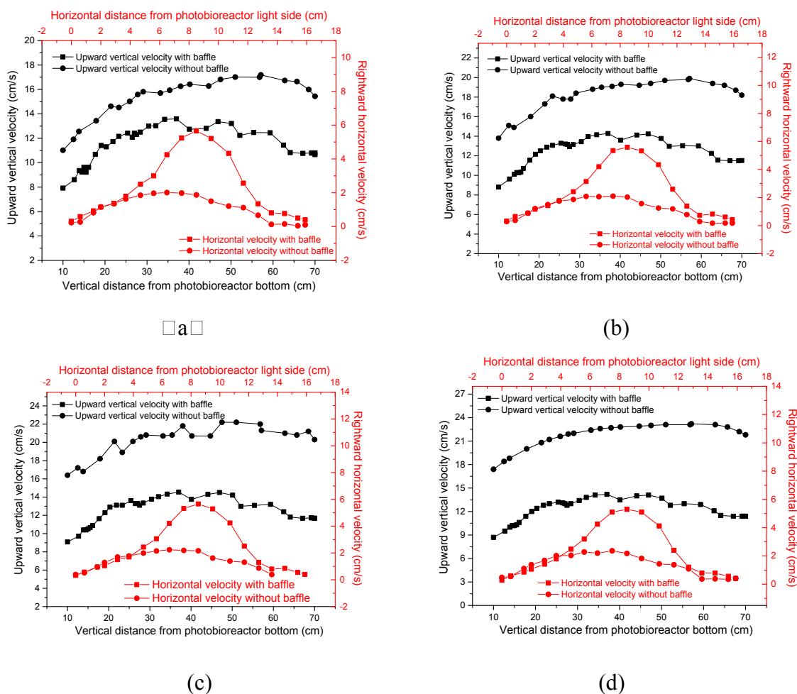
Fig.1 Vertical velocity and horizontal velocity at different position in a panel bioreactor under various gas aeration rate. (a) 0.04 vvm, (b) 0.06 vvm, (c) 0.08 vvm, (d) 0.10 vvm.
