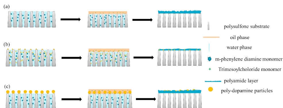
Fig. S-1. Schematic representation of (a) the conventional interfacial polymerization protocol, (b) the small poly-dopamine particles influenced interfacial polymerization protocol and (c) the big poly-dopamine particles influenced interfacial polymerization protocol
