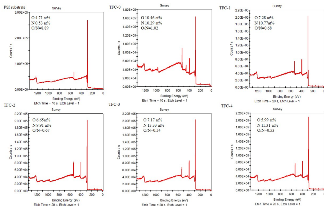
Fig. S-2. XPS spectra of PA layers on PSf substrate, TFC-0, TFC-1, TFC-2, TFC-3 and TFC-4 membrane, respectively
