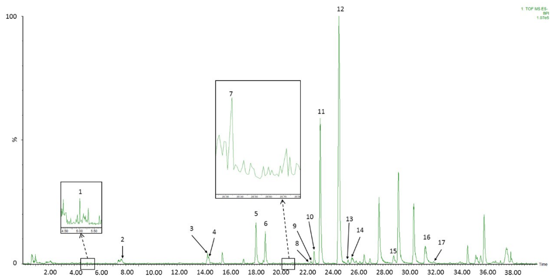
Supplementary Figure 2. Total Ion Chromatogram of Okra Seed extract (OSE) under the Negative Ion Mode
