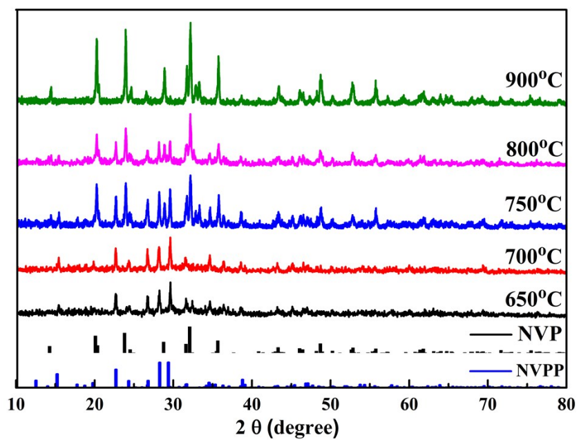
Fig. S1†. Powder XRD patterns of NVPP at different synthesis temperatures range from 650 °C to 900 °C.
