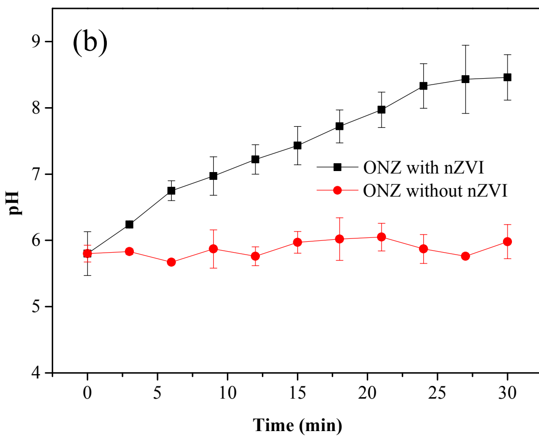
Fig. S1. Variation of TOC and ONZ concentrations (a) and pH (b) at various
