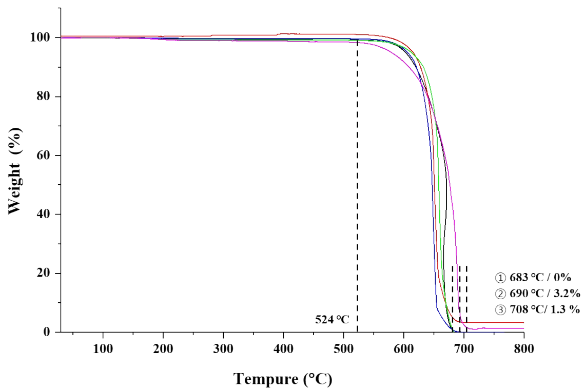
Figure 2S. TGA of CNTs prepared with various R values.
