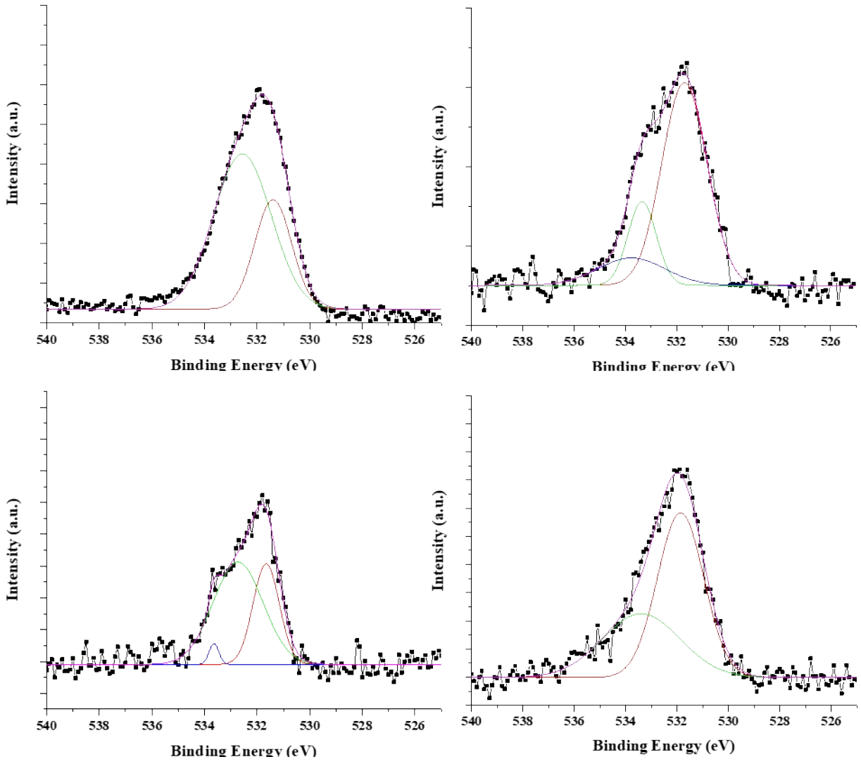
Figure 3S. O 1s XPS spectra of CNTs prepared with various R values.
