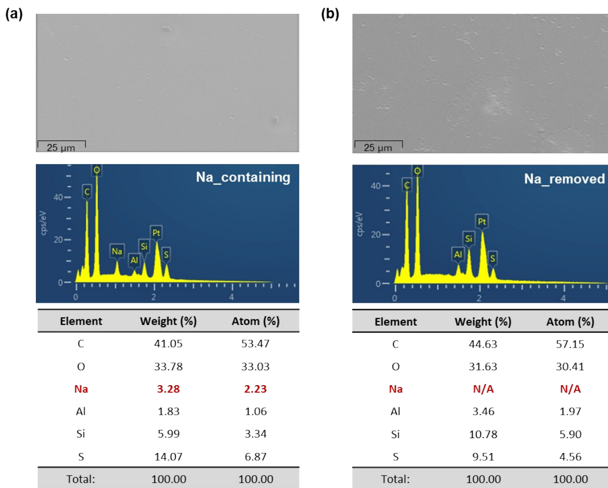
Figure S1. SEM-EDS analysis results of (a) sodium-containing and (b) sodium-removed PEDOT:PSS films on a glass substrate.
