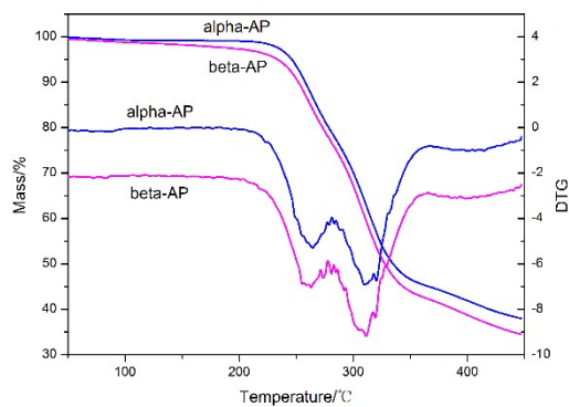
Fig.S1 TG and DTG of the two APs
