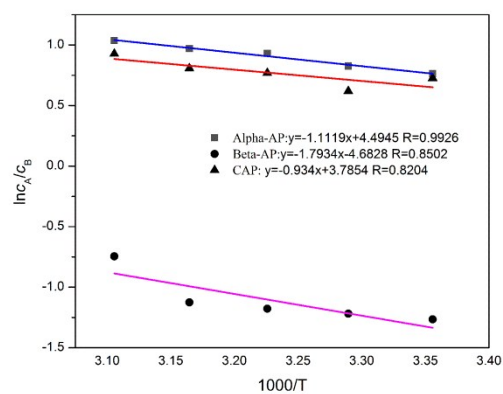
Fig.S2 Curves of \ln c_A/c_B \sim 1000/T of AZE system in 0.01M HCl medium.
