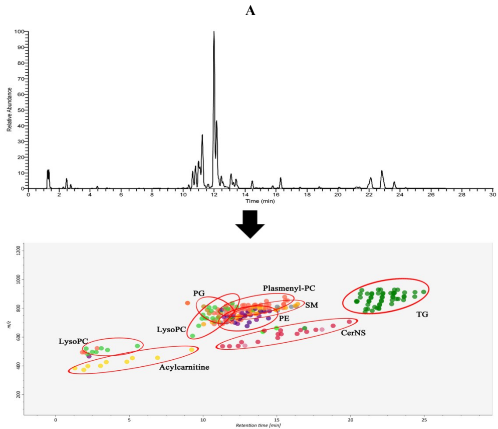
Fig. S2 Base peak chromatogram and MS/MS peak spot viewer of the total lipid fraction in MS-DIAL. (A) lung tissue ESI(+), (B) lung tissue ESI(-), (C) plasma ESI(+), and (D) plasma ESI(-).
