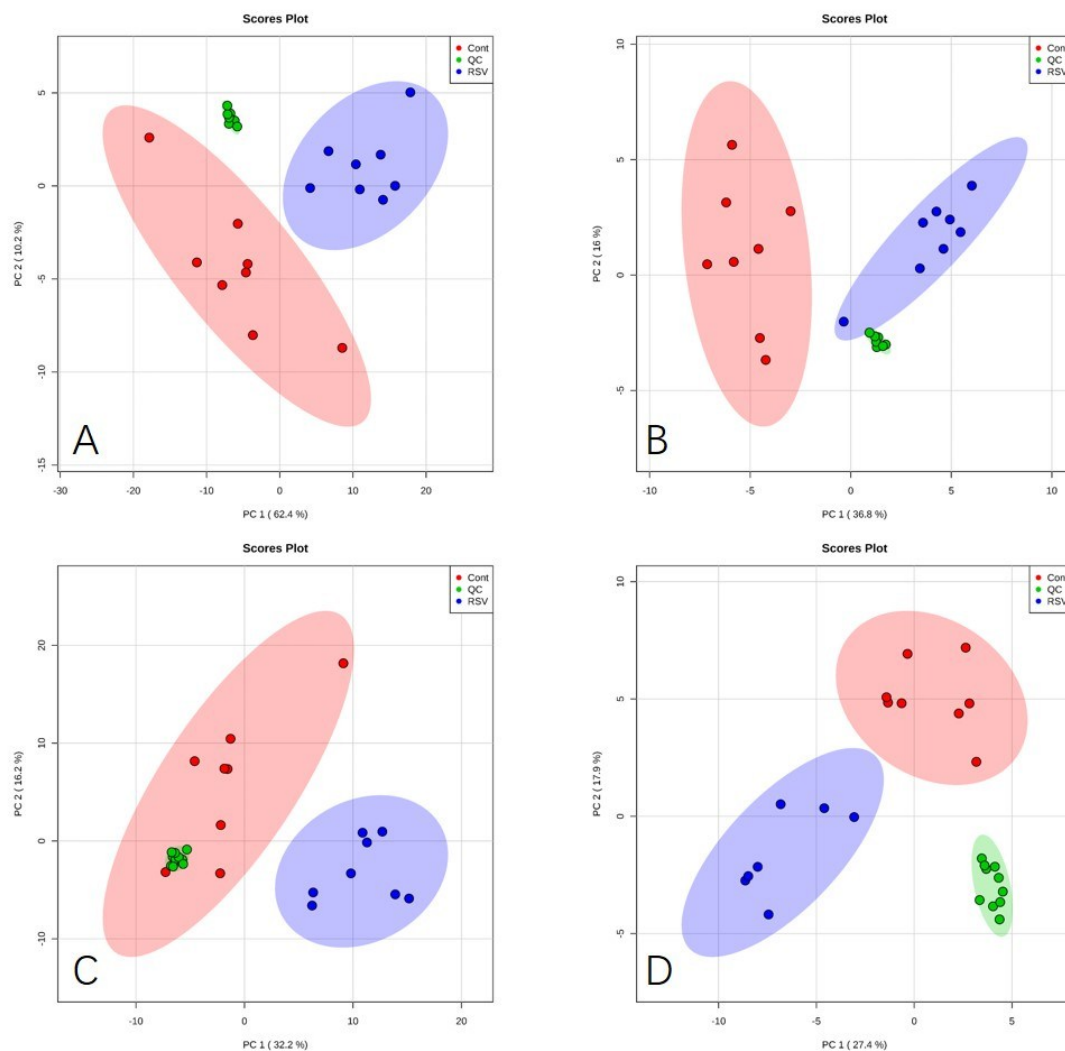
Fig. S1 The tight clustering of the QCs in the PCA scores. (A) lung tissue ESI(+), (B) lung tissue ESI(-), (C) plasma ESI(+), and (D) plasma ESI(-).
