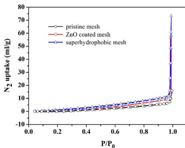
Fig. S1. N 2 adsorption-desorption isotherms at 77 K.
