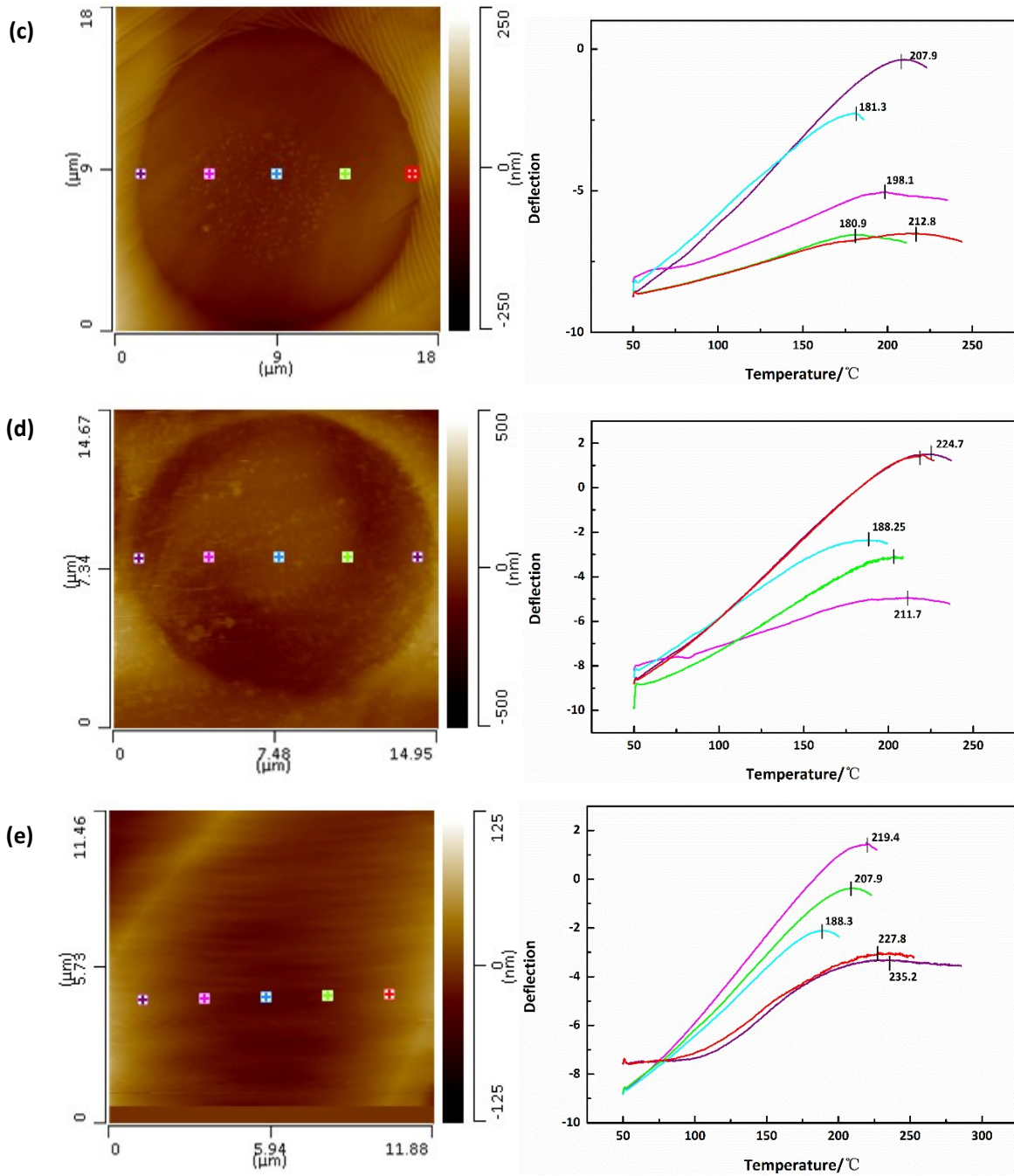
Fig.S1 (a)-(e) AFM height mapping of the cross section combined with corresponding Nano-TA measurement results for sample D2-D6.
