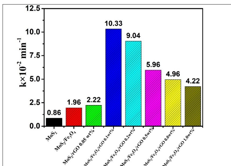
Fig. S1 The reaction rate constant ( k values) of different samples in the photocatalytic degradation of RhB.
