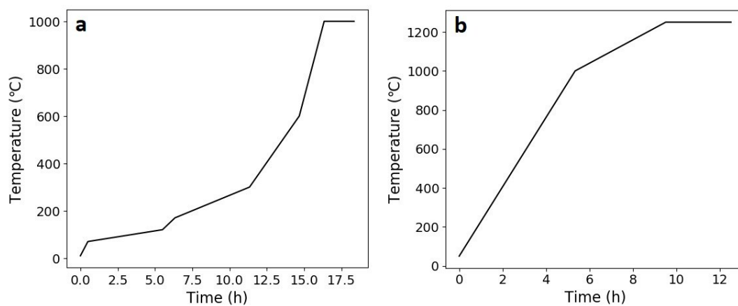
Fig. S1 (a) The temperature curve for debinding to obtain the porous glass (b) The temperature curve for sintering the porous silica glass
