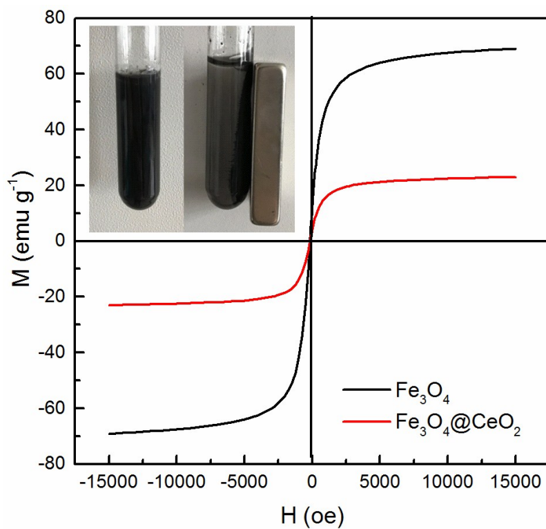
Fig. S1 Magnetization curves of \text{Fe}_3\text{O}_4 and \text{Fe}_3\text{O}_4@\text{CeO}_2 at room temperature.
