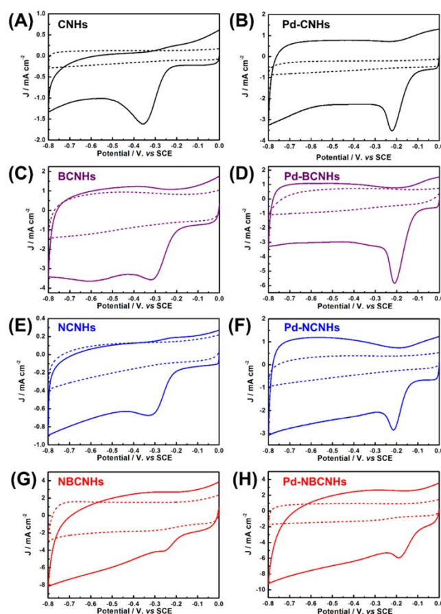
Fig. S1 CV curves of (A) CNHs, (B) Pd-CNHs, (C) BCNHs, (D) Pd-BCNHs, (E) NCNHs, (F) Pd-NCNHs, (G) NBCNHs and (H) Pd-NBCNHs at a scan rate of 50 mV s -1 in O 2 -saturated (solid line) or N 2 -saturated (dash line) 0.1 M KOH solution.
