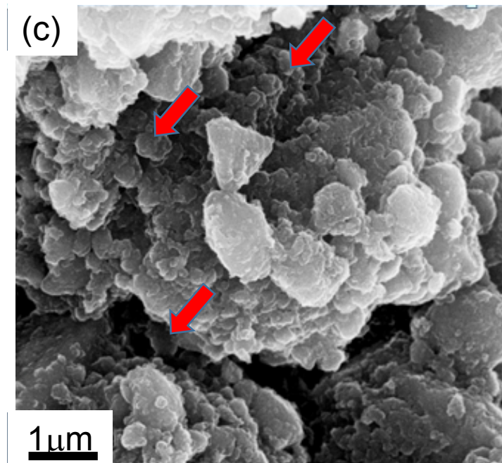
Fig.S3 Co-milled with PP for 3h with higher magnification. The dark particles marked by the arrows correspond to the dark dots shown in Fig. S2(b).which might be associated with carbon species, although further confirmation is needed.
