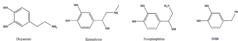
Fig. S1. The chemical structures of the dopamine (DA), epinephrine (E), norepinephrine (NE) and 3,4-dihydroxybenzylamine (DHBA)
