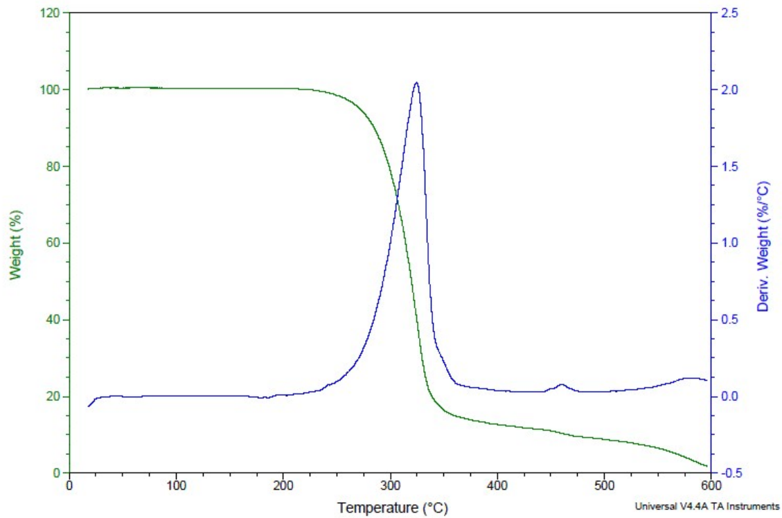
Figure 2: Thermogravimetric analysis (TGA) thermogram of 110
