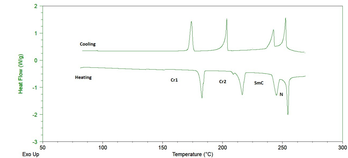
Figure 1: DSC curve of I10 at heating rate 10 °C/min for heating and cooling cycles.
