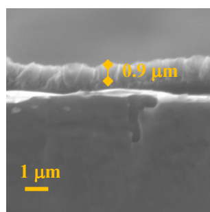
Fig. S2 The Cross-section SEM image of the Al@MnO 2 prepared at 18 h.
