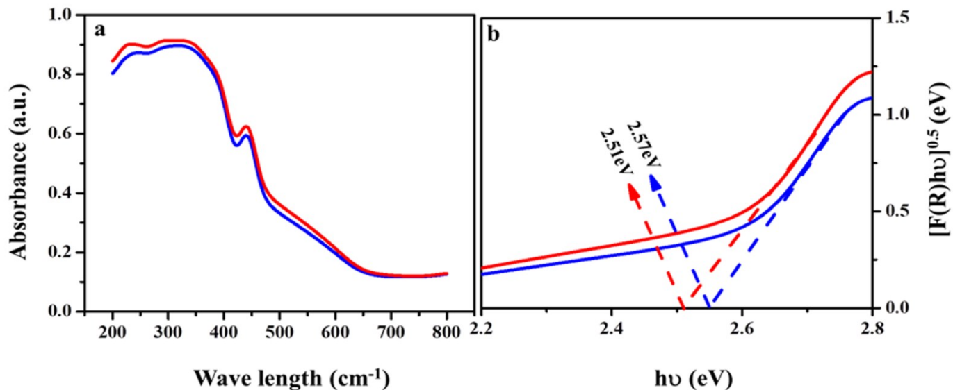
Figure: S1 (a, b) UV spectrum of (a) MIL-53(Fe)- hydrated and (b) MIL-53(Fe)- dehydrated , (Right side) Kubelka-Munk plot illustrating the band gap energy for MIL-53(Fe)- hydrated and (b) MIL-53(Fe)-dehydrated.
