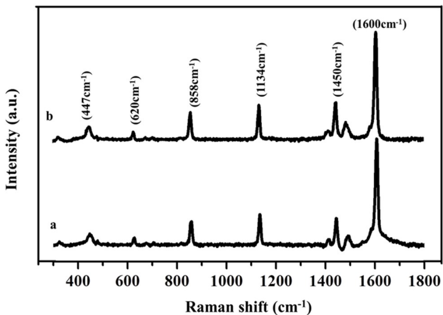
Figure: S2 (a, b) Raman spectra of (a) MIL-53(Fe)- hydrated and (b) MIL-53(Fe)- dehydrated
