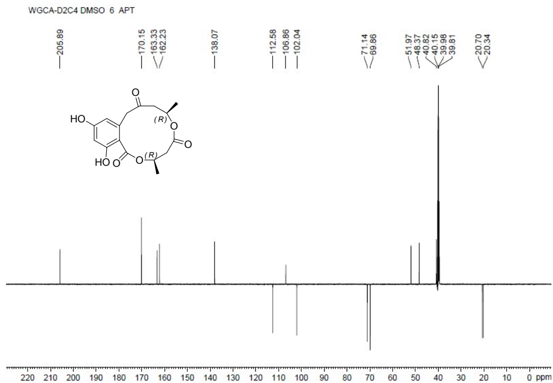
Figure S12-4. APT Spectrum of Compound 12
