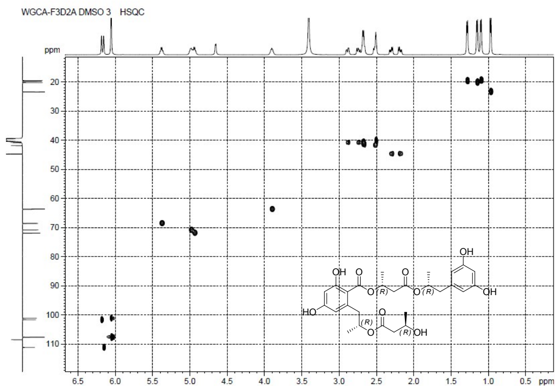
Figure S10-6. HSQC Spectrum of Compound 10
