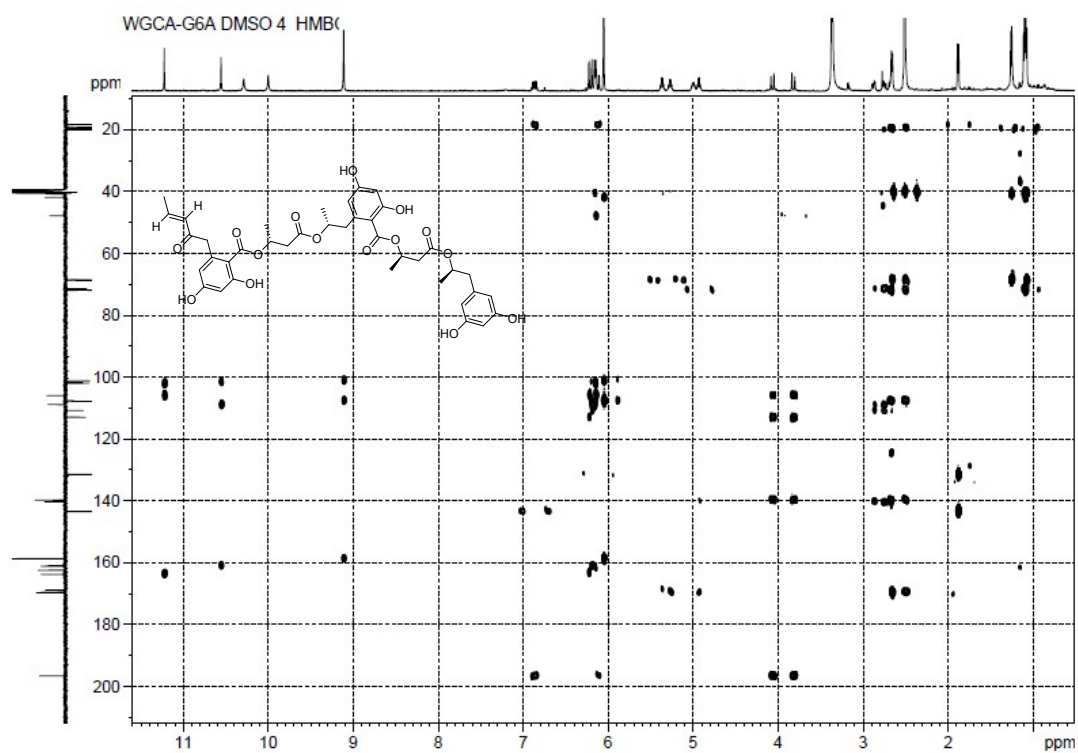
Figure S2-7. HMBC Spectrum of Compound 2
