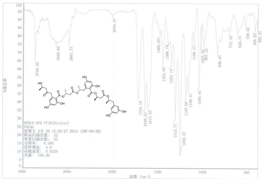
Figure S5-2. IR Spectrum of Compound 5
