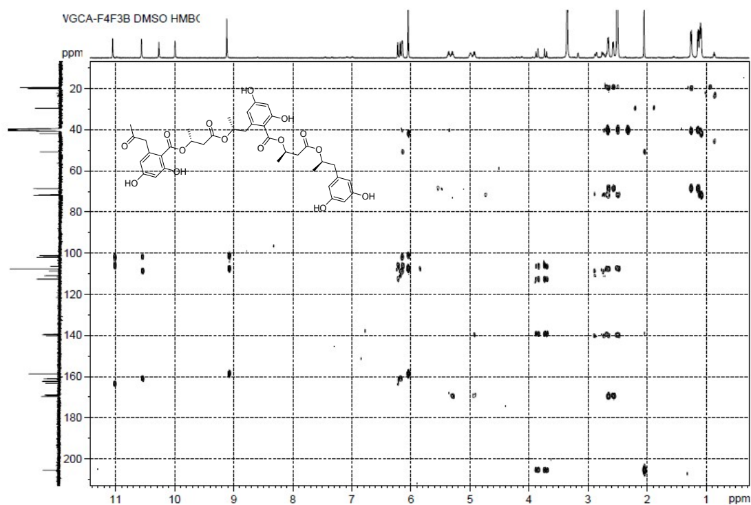
Figure S4-7. HMBC Spectrum of Compound 4
