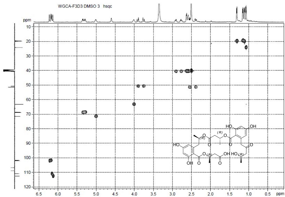
Figure S9-6. HSQC Spectrum of Compound 9
