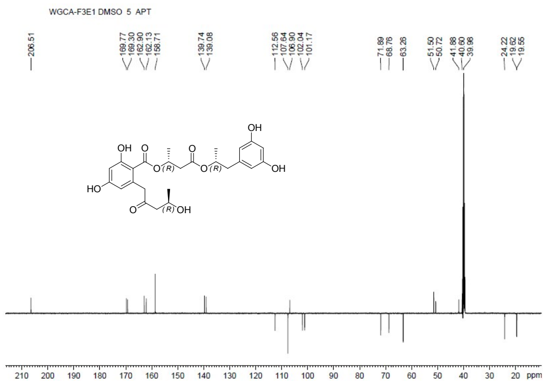
Figure S11-4. 13 C-NMR Spectrum of Compound 11
