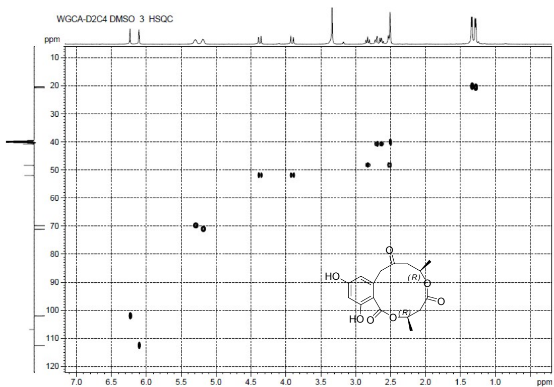
Figure S12-6. HSQC Spectrum of Compound 12
