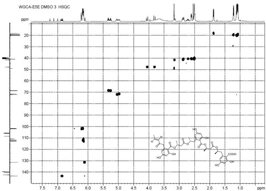
Figure S3-6. HSQC Spectrum of Compound 3
