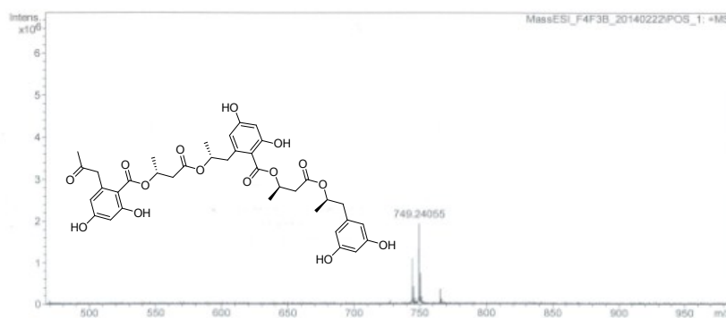
Figure S4-1. HRESIMS Spectrum of Compound 4
