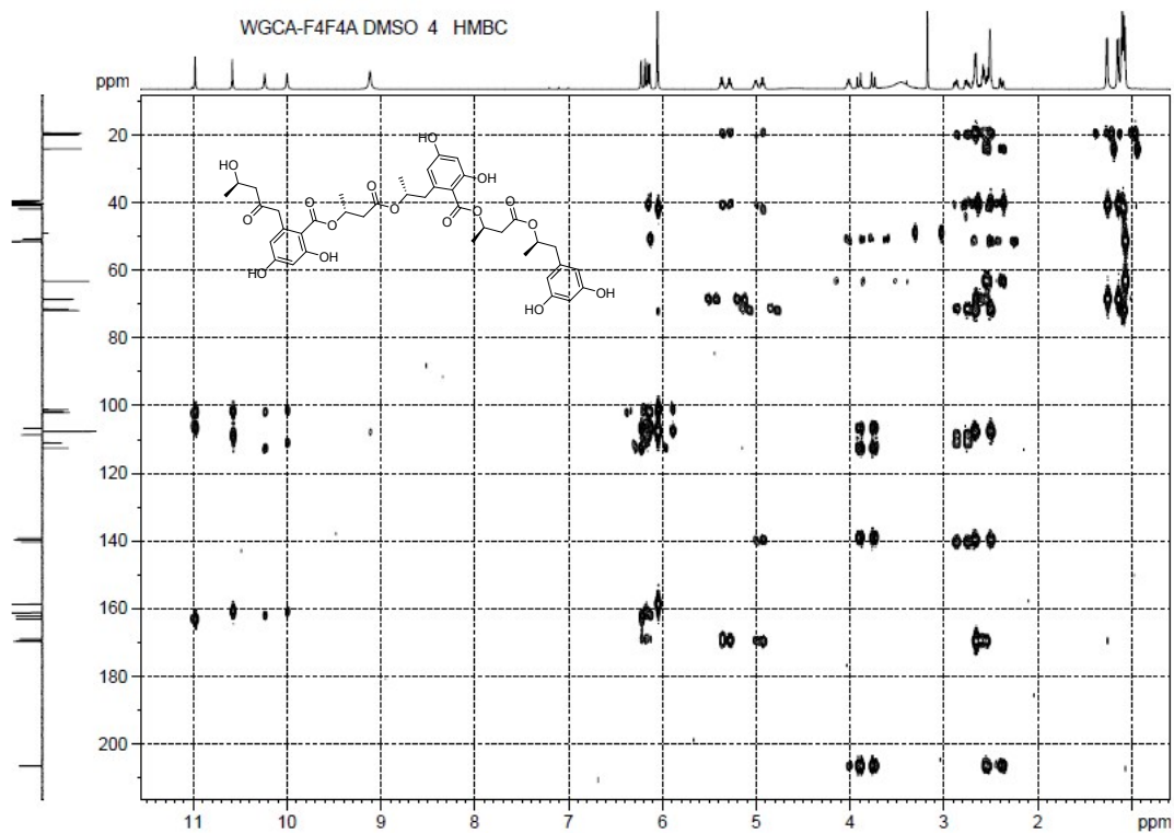
Figure S5-7. HMBC Spectrum of Compound 5
