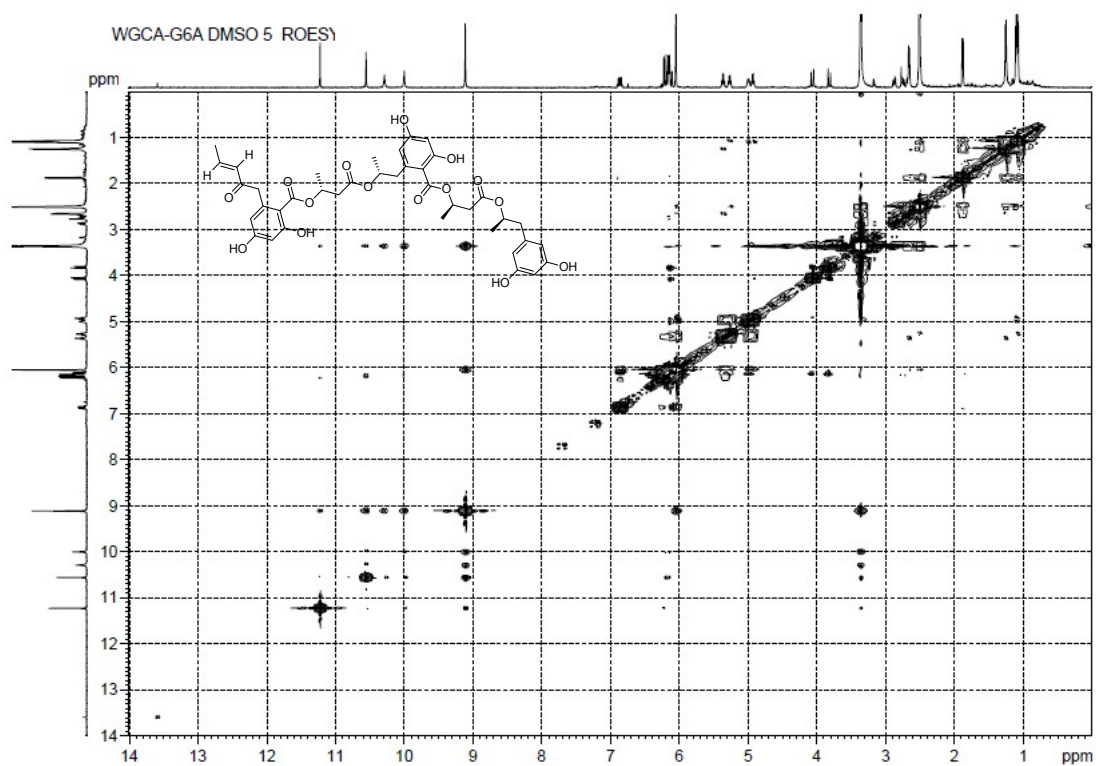
Figure S2-8. ROESY Spectrum of Compound 2
