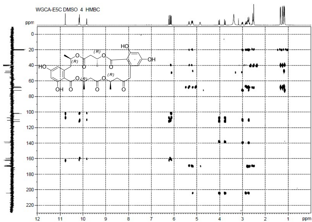
Figure S8-7. HMBC Spectrum of Compound 8
