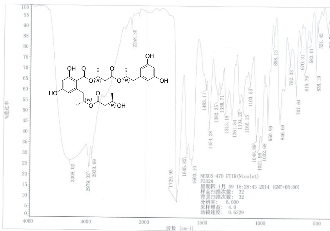
Figure S10-2. IR Spectrum of Compound 10
