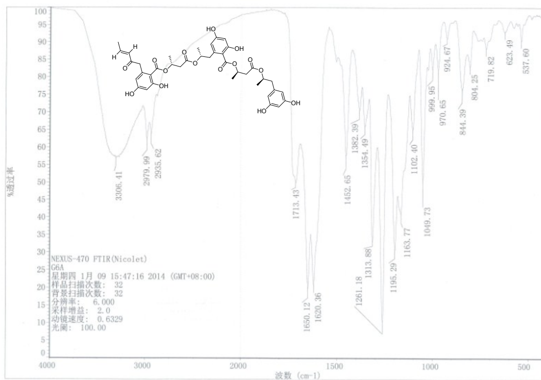
Figure S2-2. IR Spectrum of Compound 2
