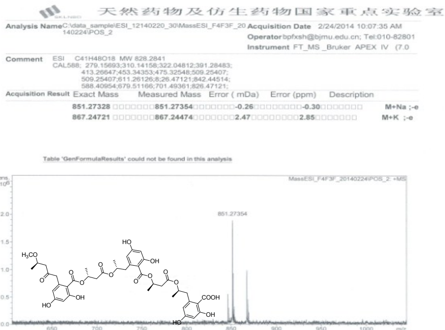
Figure S7-1. HRESIMS Spectrum of Compound 7
