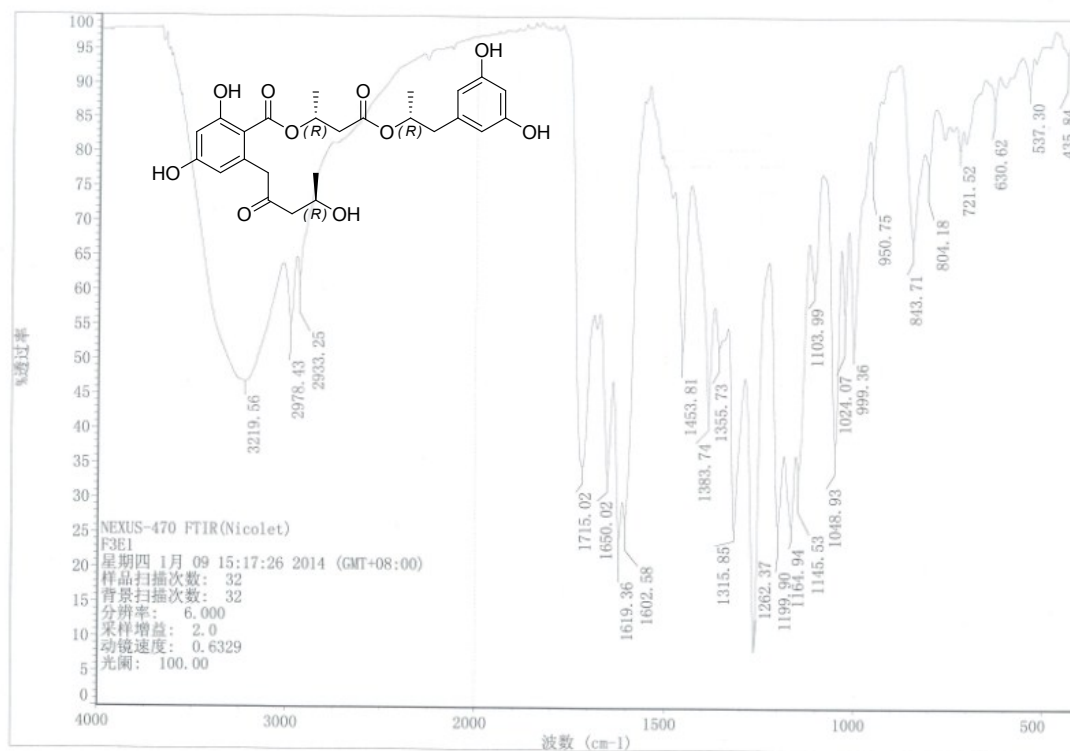
Figure S11-2. IR Spectrum of Compound 11
