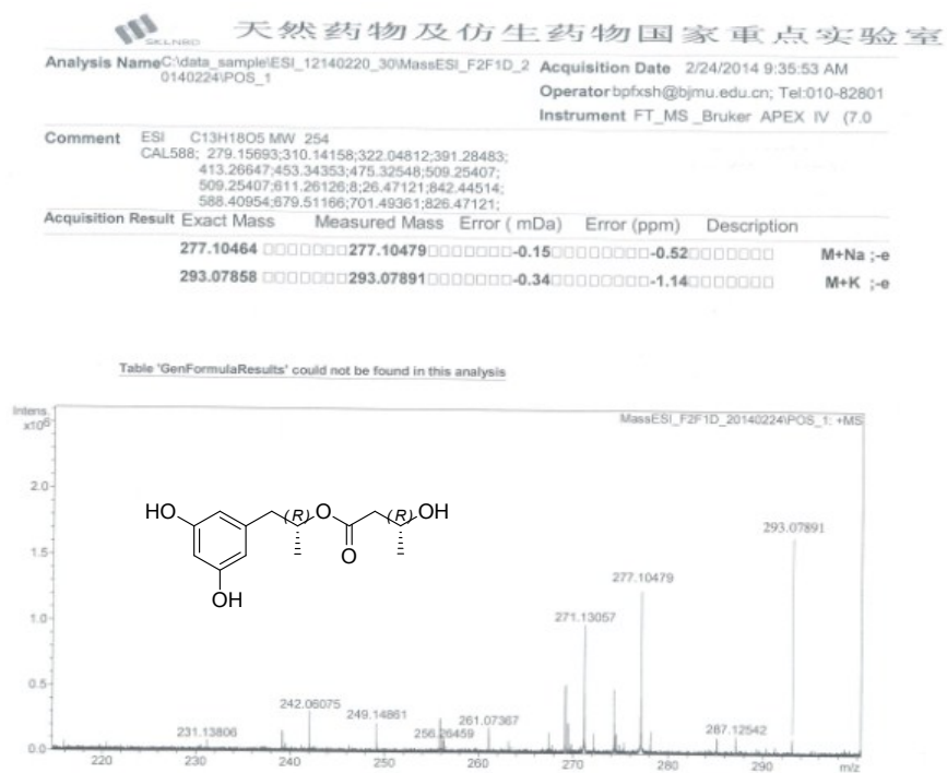
Figure S13-1. HRESIMS Spectrum of Compound 13
