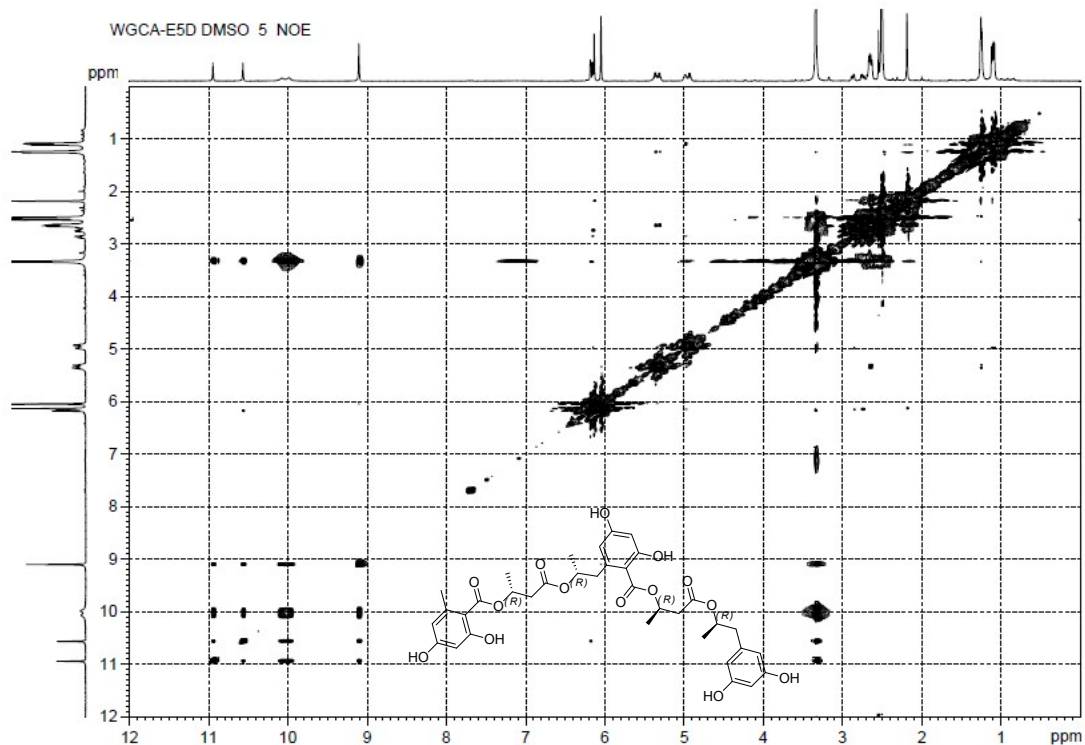
Figure S1-8. NOESY Spectrum of Compound 1
