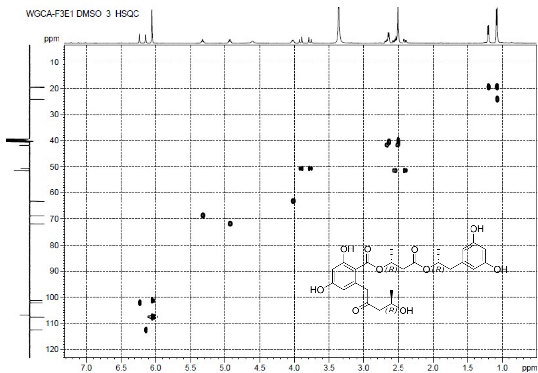
Figure S11-6. HSQC Spectrum of Compound 11
