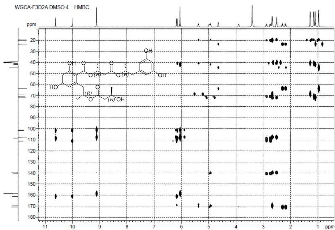
Figure S10-7. HMBC Spectrum of Compound 10
