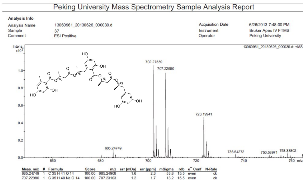
Figure S1-1. HRESIMS Spectrum of Compound 1
