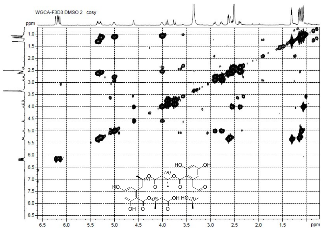
Figure S9-5. COSY Spectrum of Compound 9
