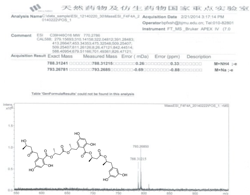
Figure S5-1. HRESIMS Spectrum of Compound 5
