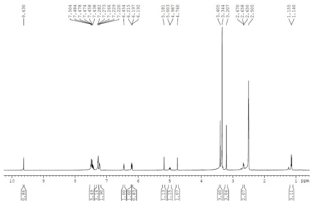
Figure Sb-3. 1 H-NMR Spectrum of ( R )MPA ester of 1d
