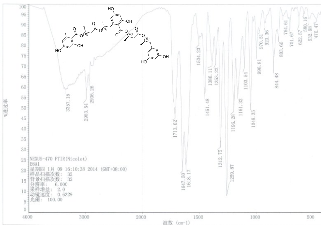
Figure S1-2. IR Spectrum of Compound 1
