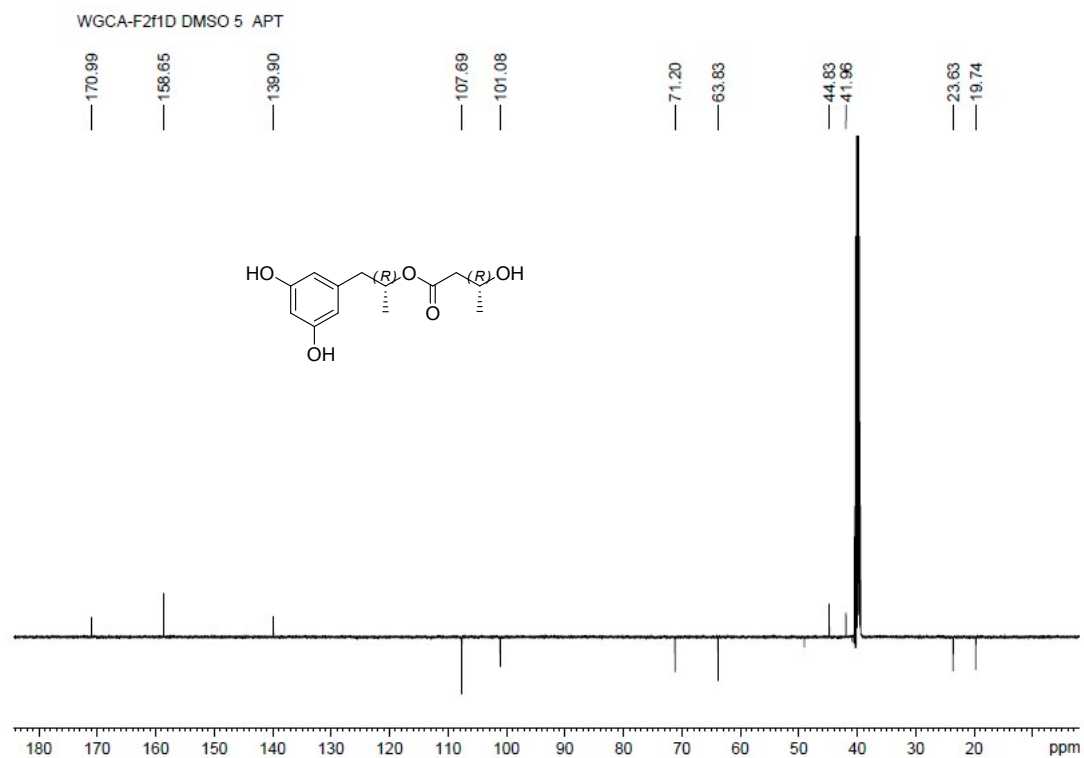
Figure S13-4. APT Spectrum of Compound 13
