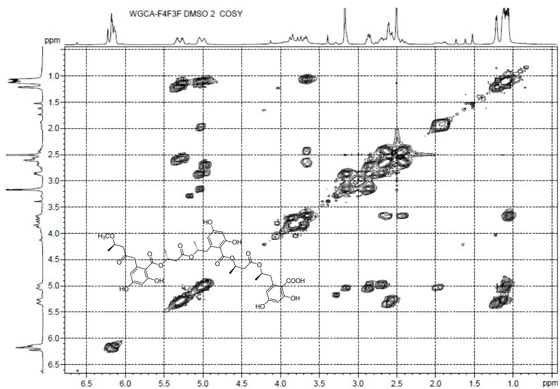
Figure S7-5. COSY Spectrum of Compound 7
