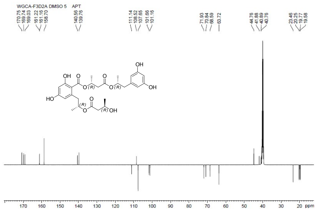
Figure S10-4. APT Spectrum of Compound 10
