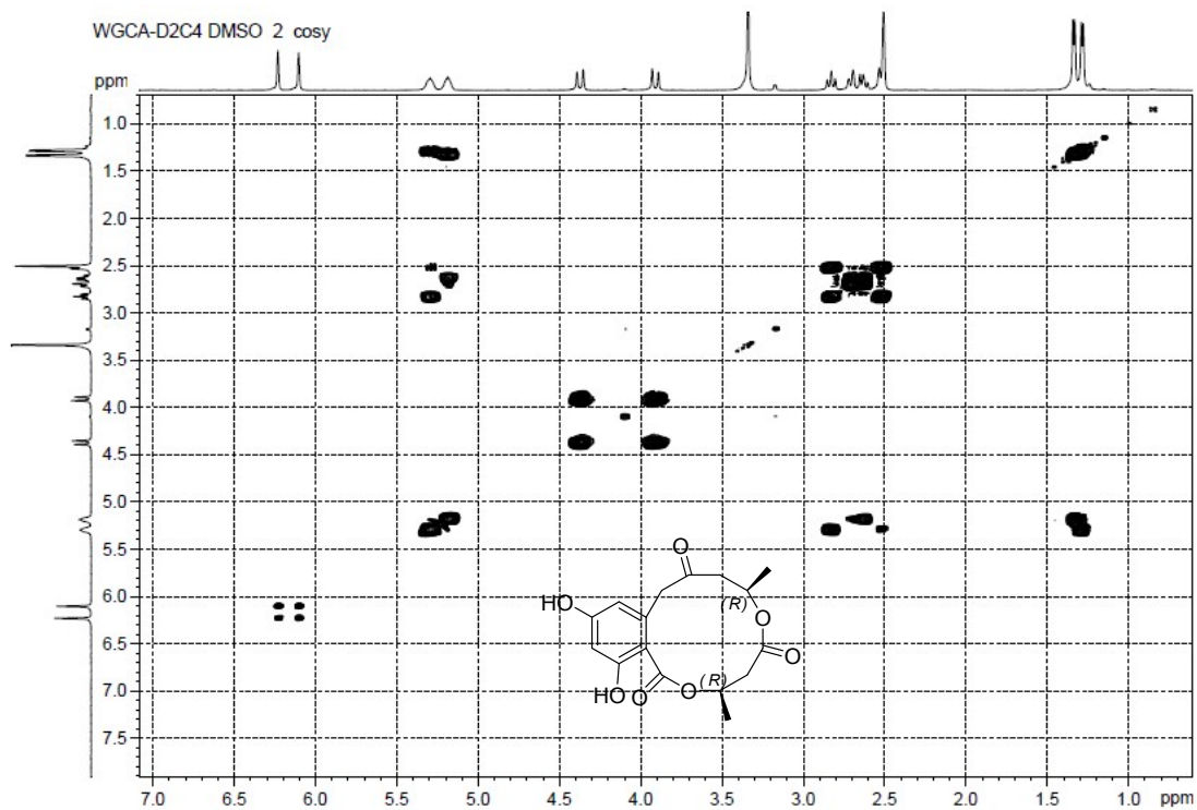
Figure S12-5. COSY Spectrum of Compound 12
