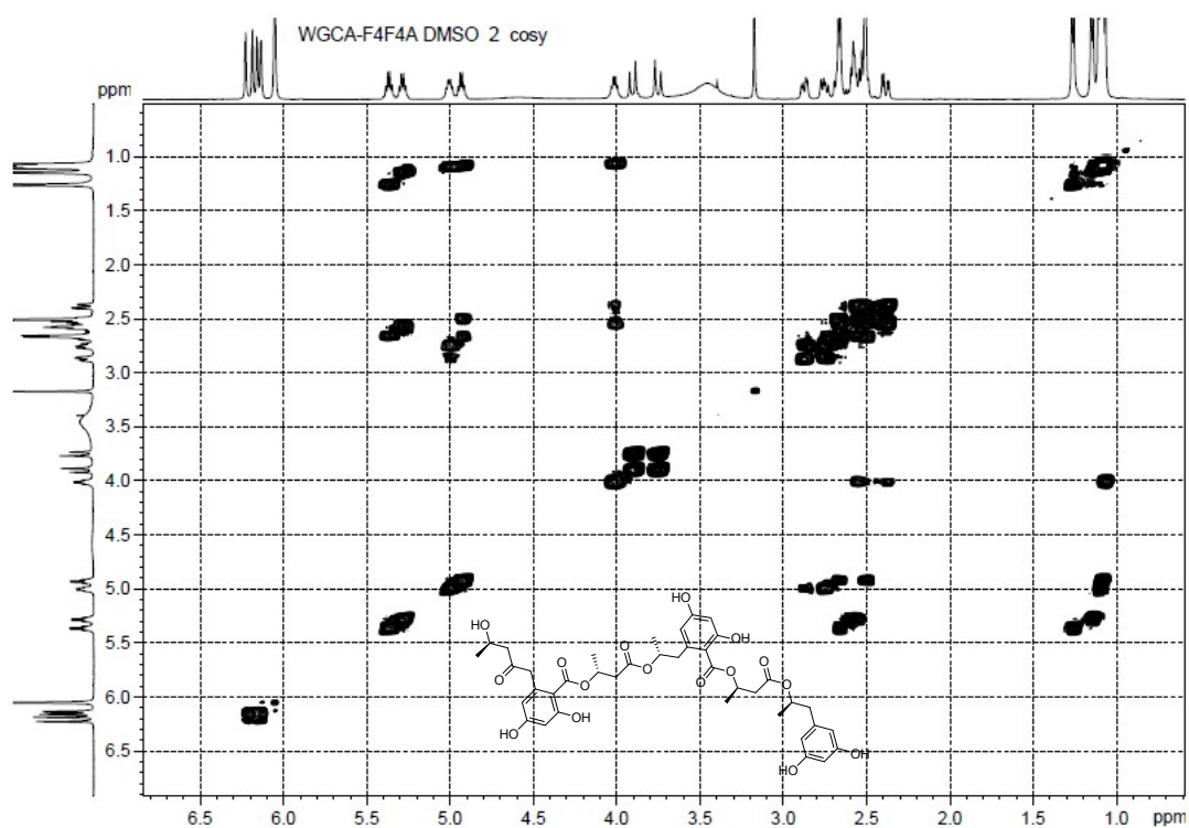
Figure S5-5. COSY Spectrum of Compound 5
