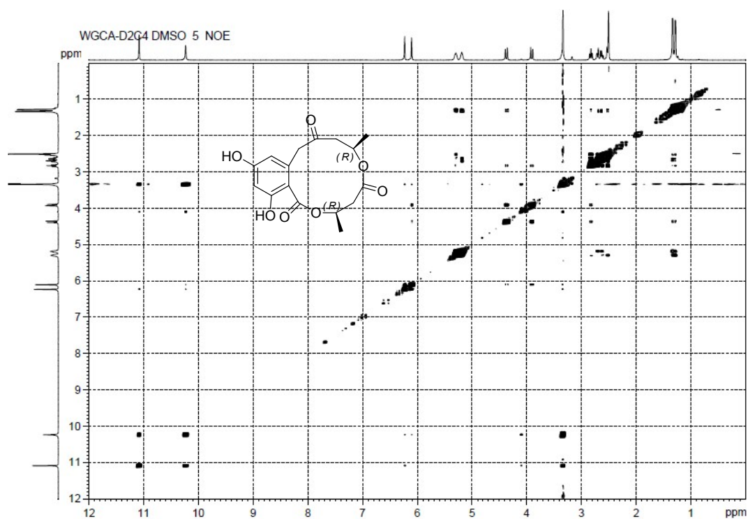
Figure S12-8. NOESY Spectrum of Compound 14
