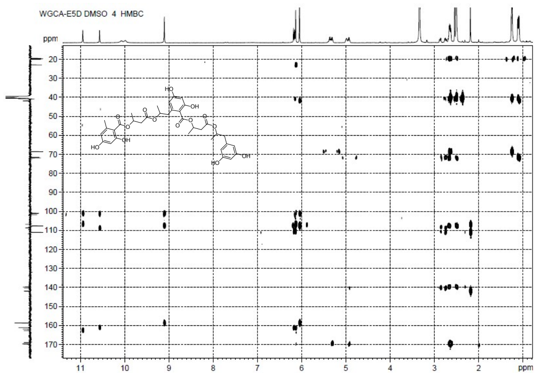
Figure S1-7. HMBC Spectrum of Compound 1
