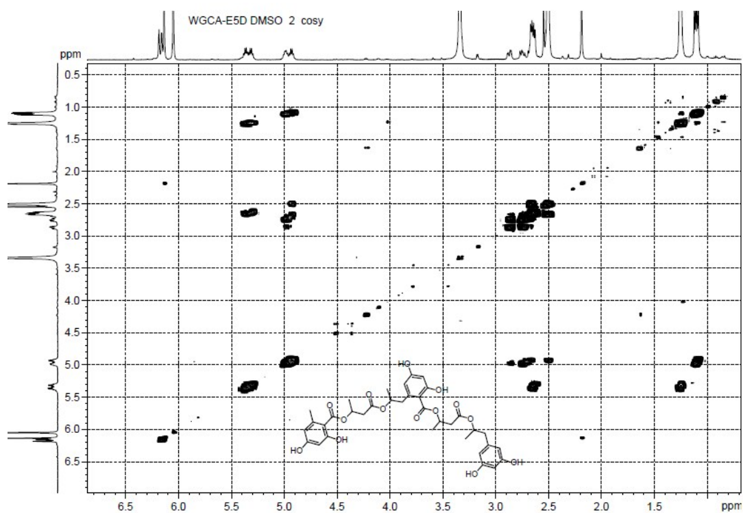
Figure S1-5. COSY Spectrum of Compound 1
