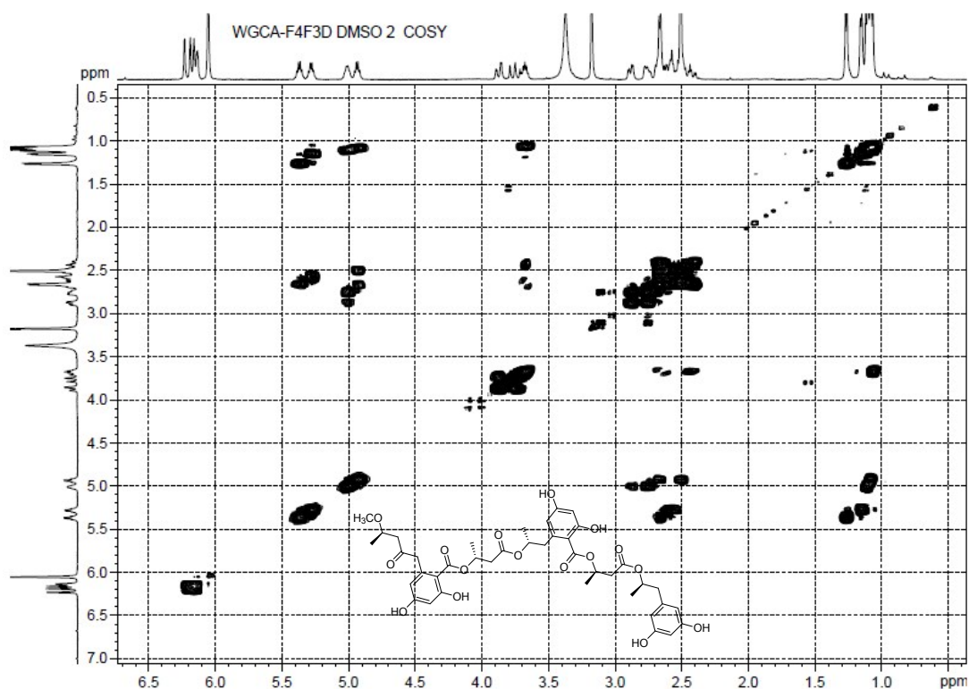
Figure S6-5. COSY Spectrum of Compound 6
