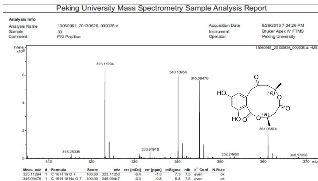
Figure S12-1. HRESIMS Spectrum of Compound 12
