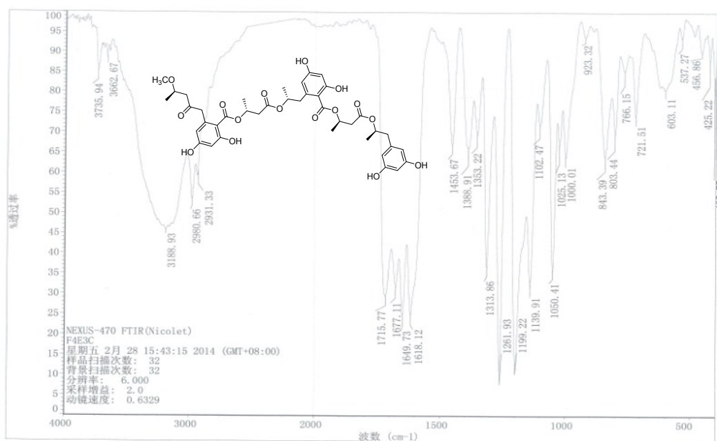
Figure S6-2. IR Spectrum of Compound 6
