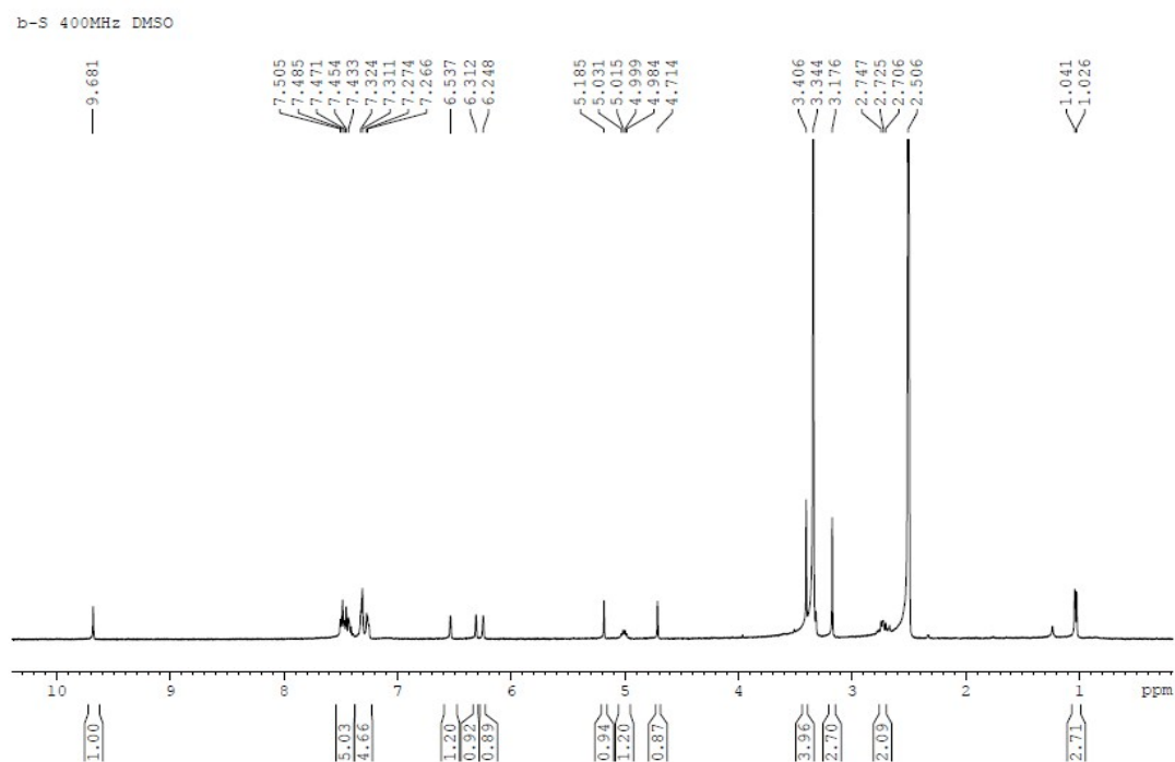
Figure Sb-2. 1 H-NMR Spectrum of (S)MPA ester of 1d
