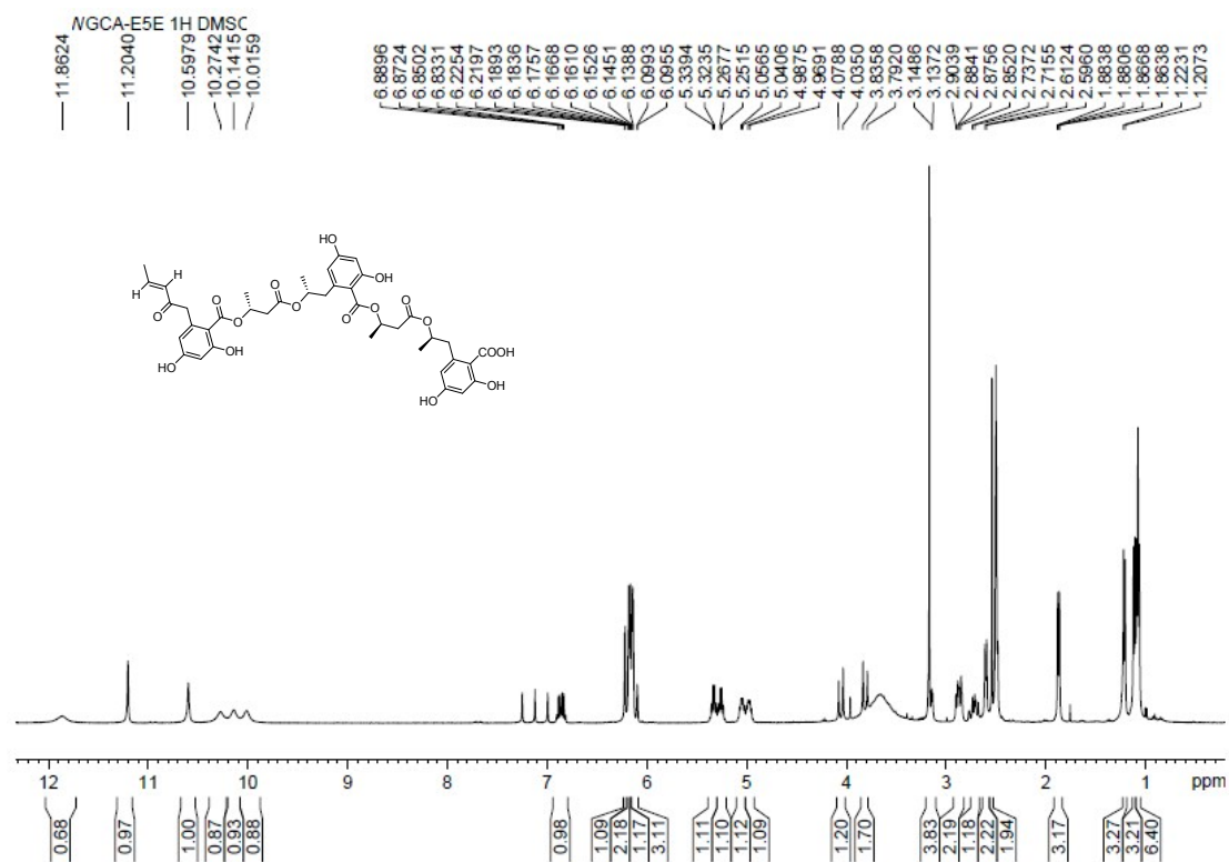
Figure S3-3. 1 H-NMR Spectrum of Compound 3
