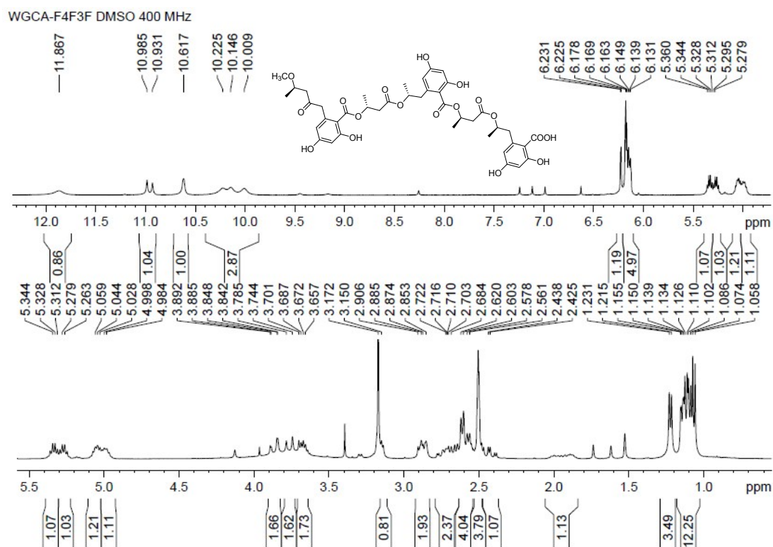
Figure S7-3. ¹H-NMR Spectrum of Compound 7
