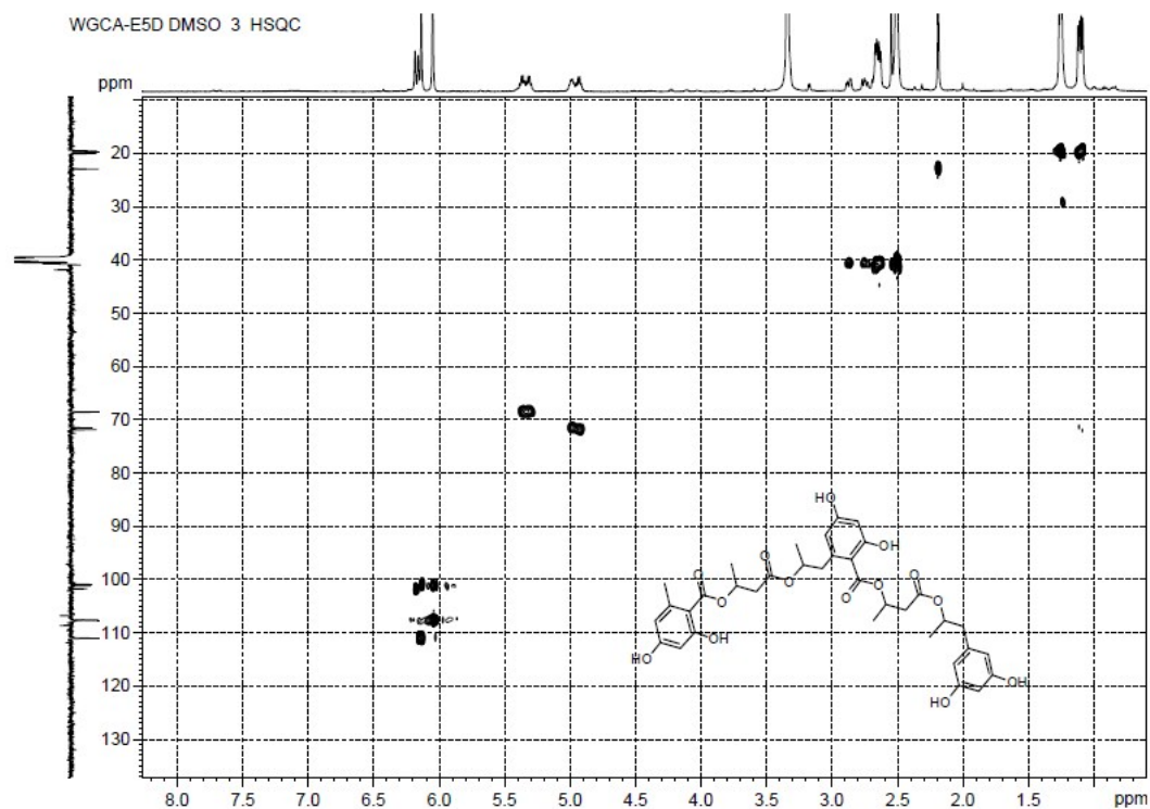
Figure S1-6. HSQC Spectrum of Compound 1
