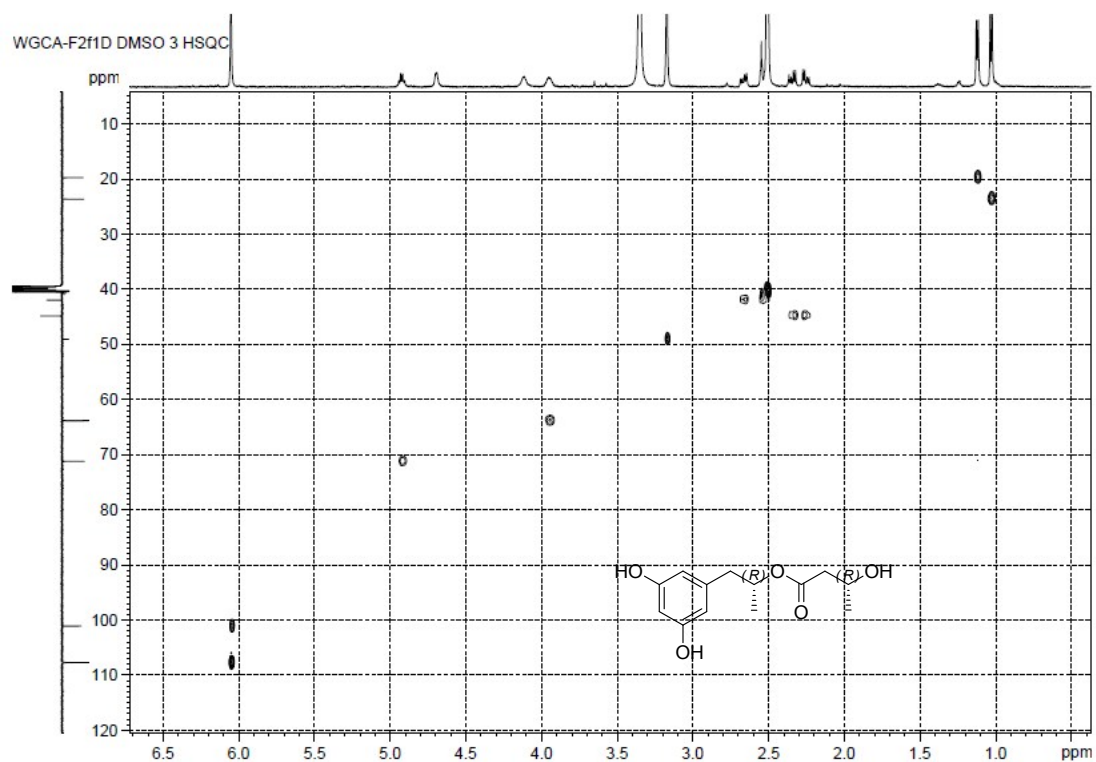
Figure S13-6. HSQC Spectrum of Compound 13
