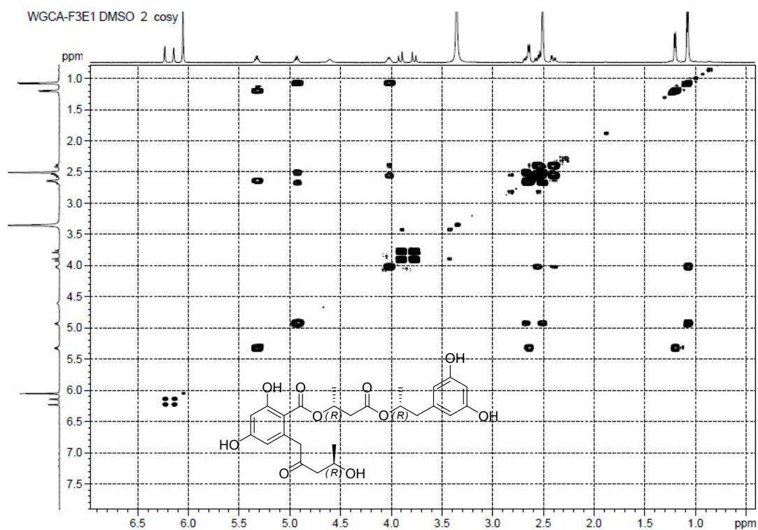
Figure S11-5. COSY Spectrum of Compound 11
