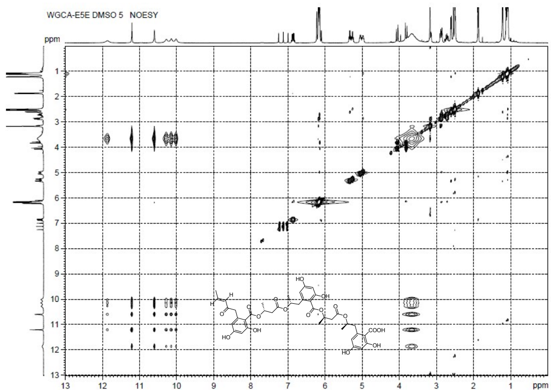
Figure S3-8. ROESY Spectrum of Compound 3
