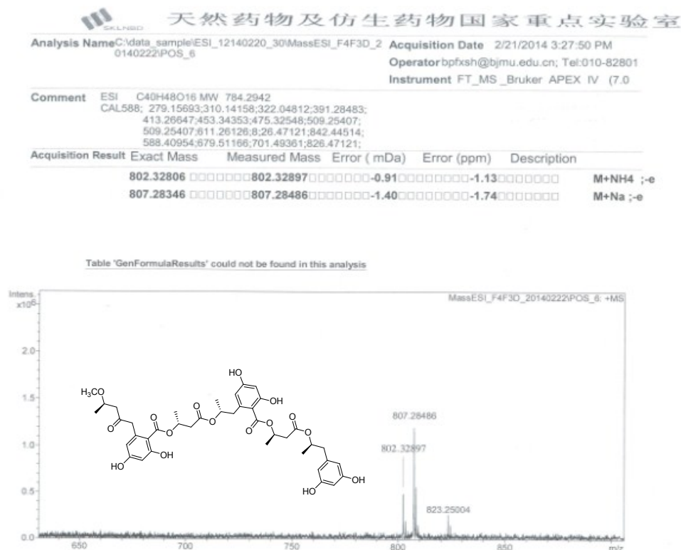
Figure S6-1. HRESIMS Spectrum of Compound 6
