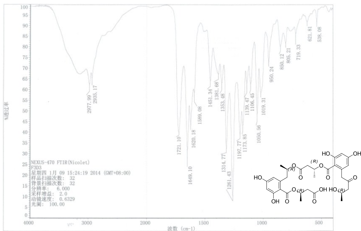
Figure S9-2. IR Spectrum of Compound 9
