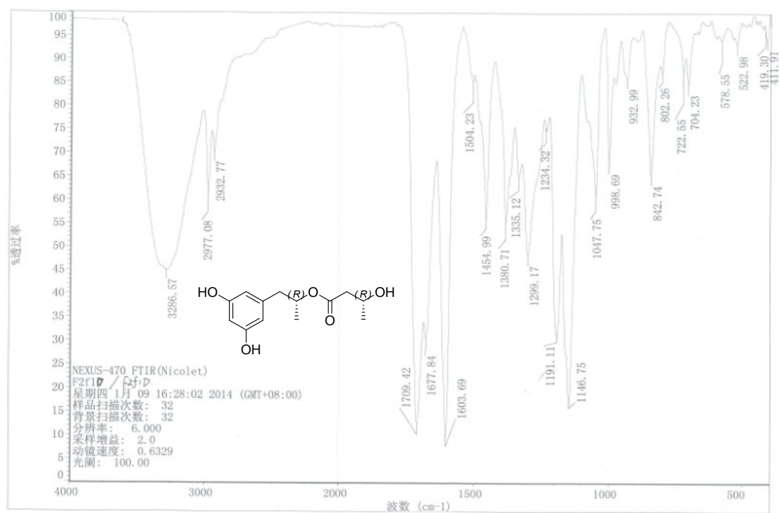
Figure S13-2. IR Spectrum of Compound 13
