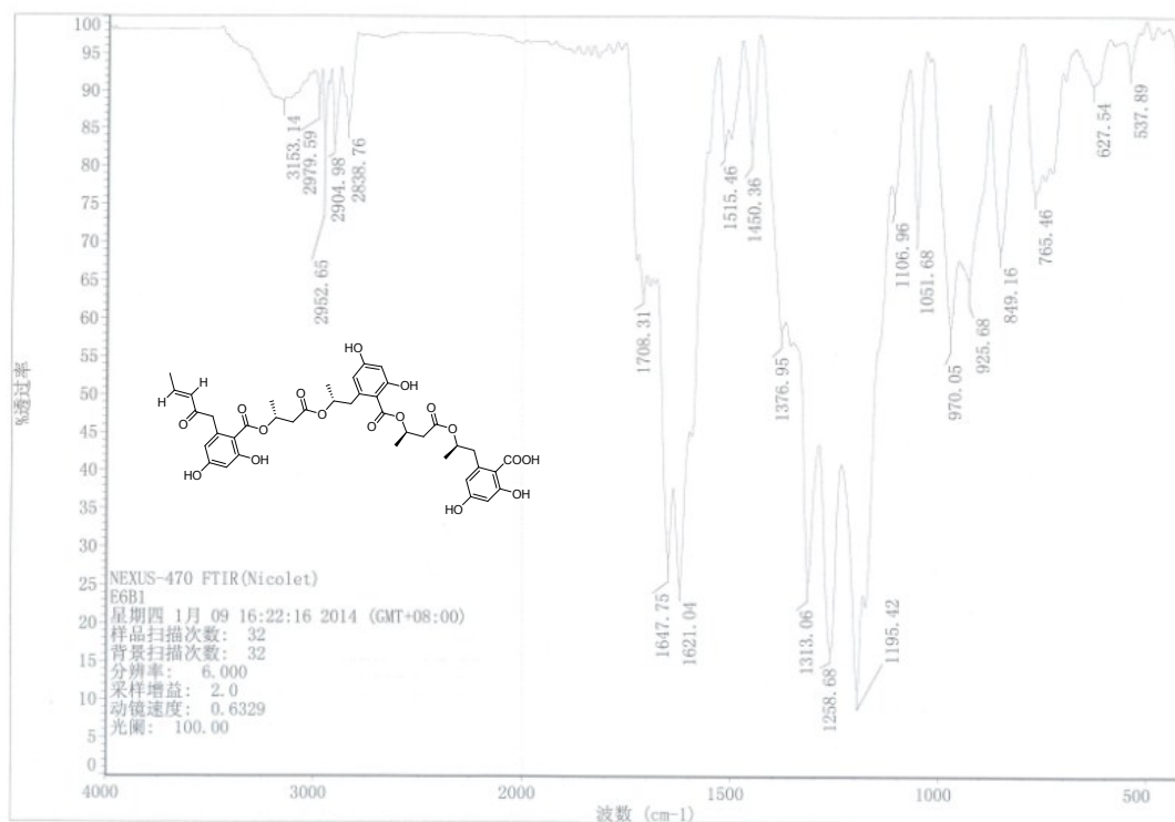
Figure S3-2. IR Spectrum of Compound 3
