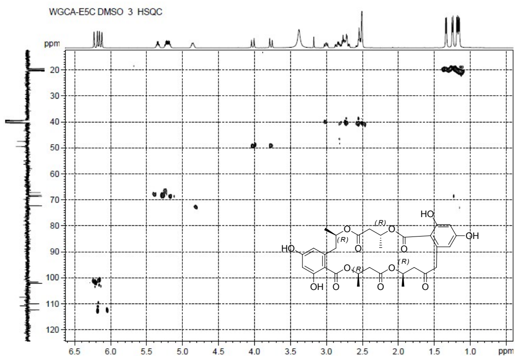
Figure S8-6. HSQC Spectrum of Compound 8
