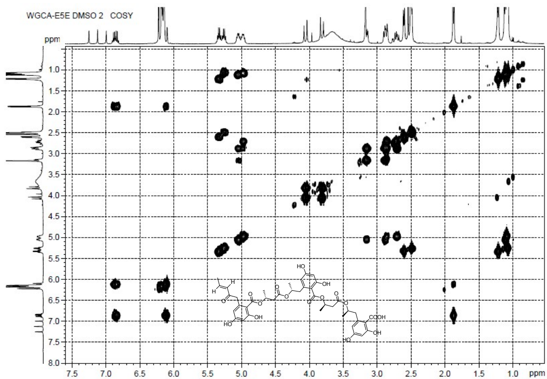
Figure S3-5. COSY Spectrum of Compound 3
