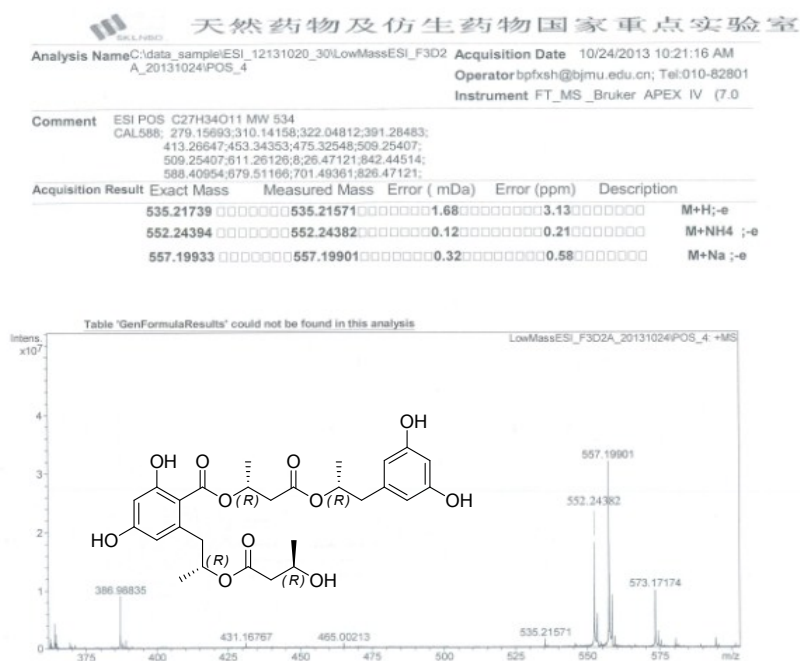
Figure S10-1. HRESIMS Spectrum of Compound 10
