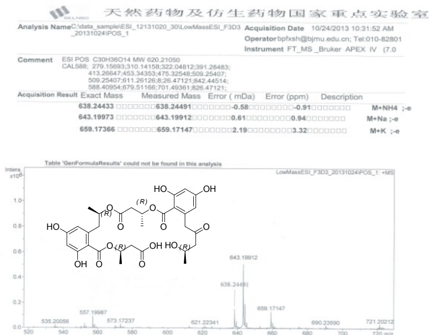
Figure S9-1. HRESIMS Spectrum of Compound 9
