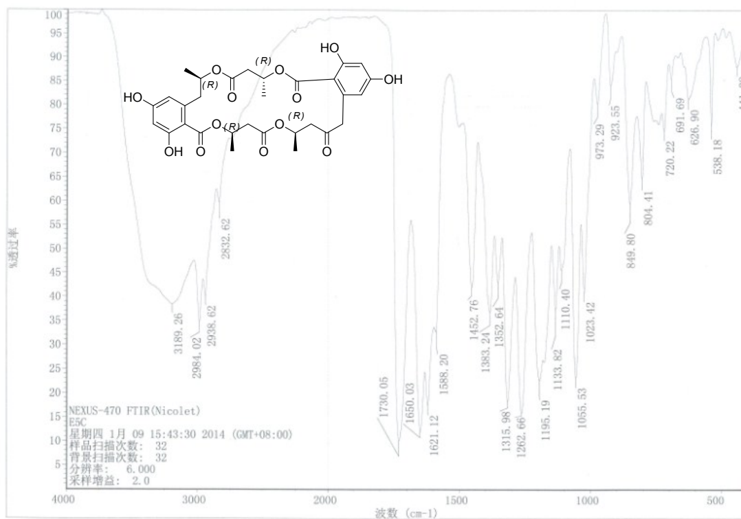
Figure S8-2. IR Spectrum of Compound 8
