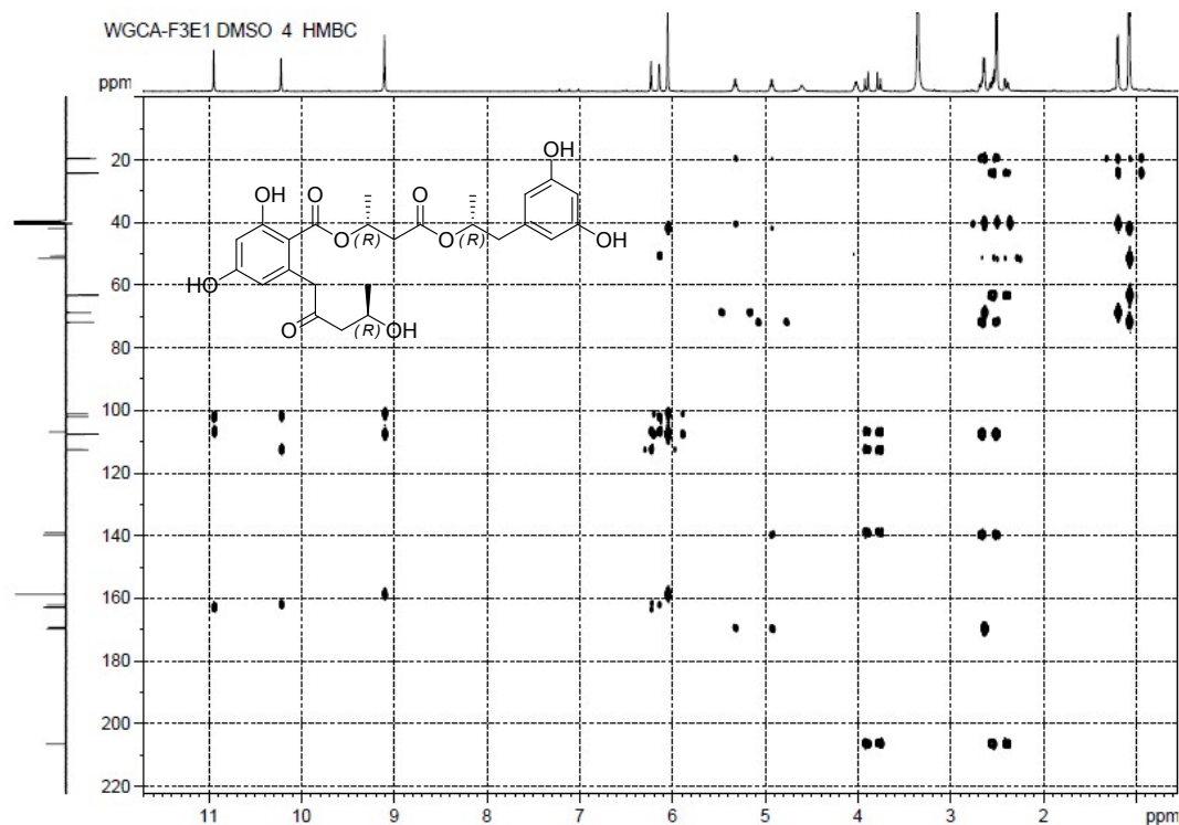
Figure S11-7. HMBC Spectrum of Compound 11
