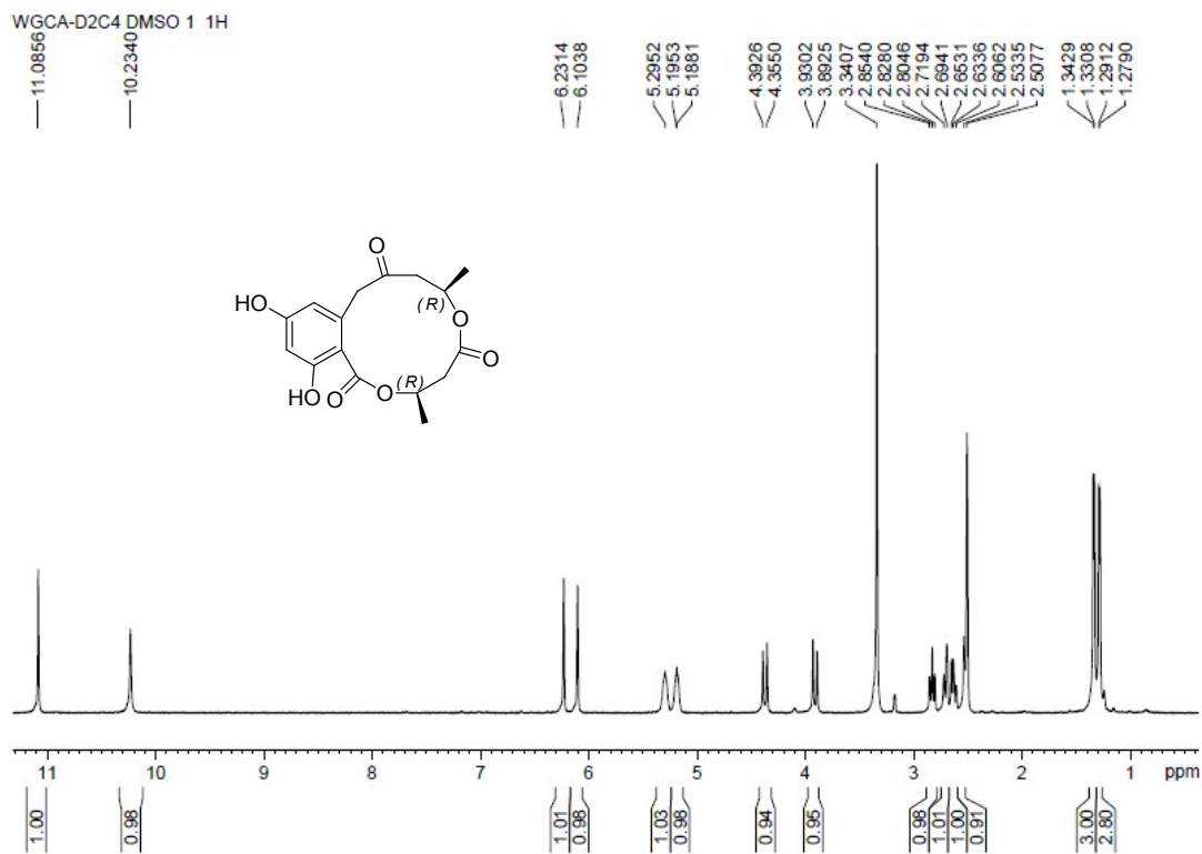
Figure S12-3. 1 H-NMR Spectrum of Compound 12
