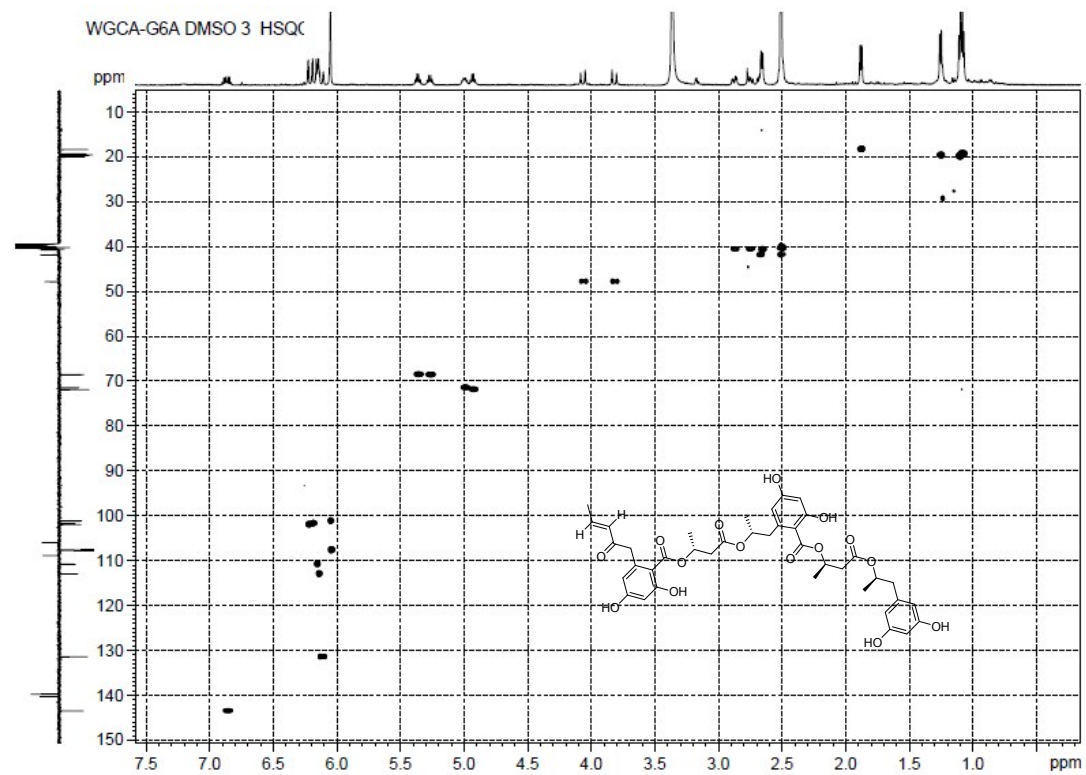
Figure S2-6. HSQC Spectrum of Compound 2
