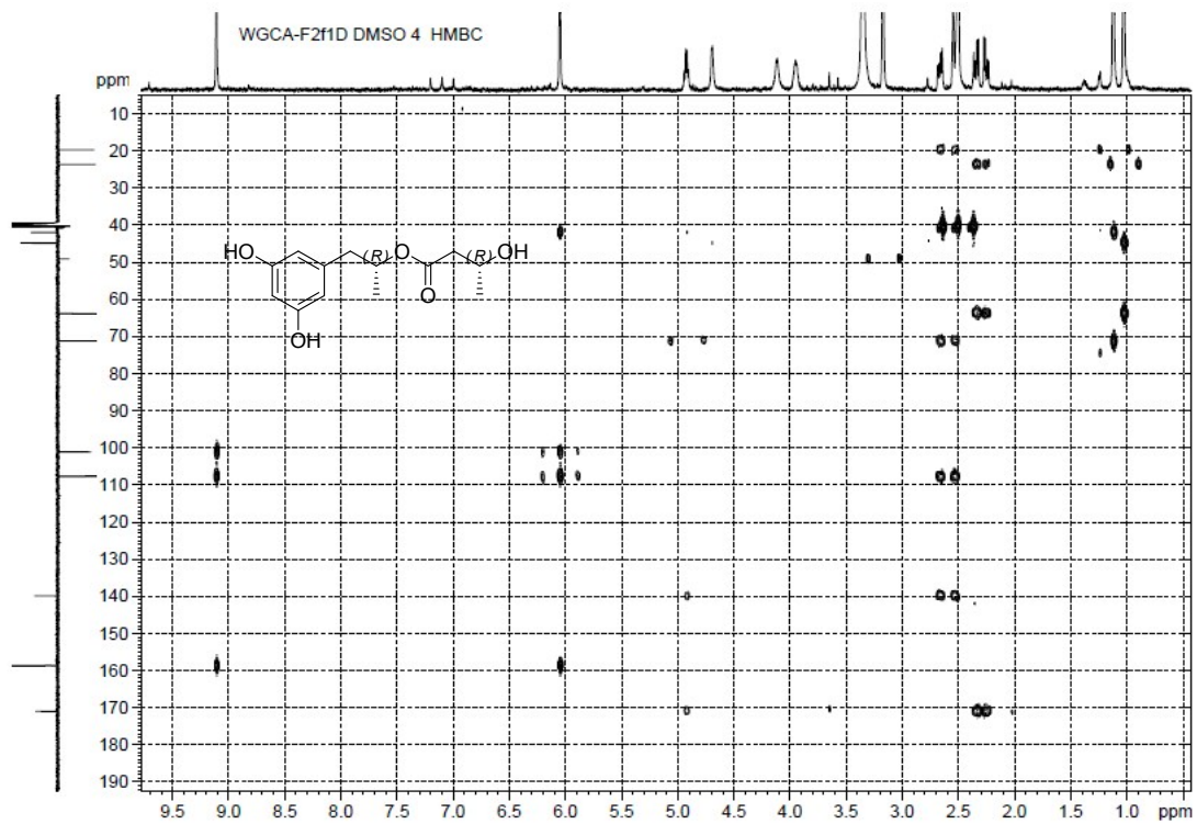
Figure S13-7. HMBC Spectrum of Compound 13
