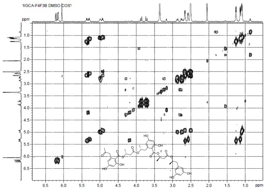
Figure S4-5. COSY Spectrum of Compound 4
