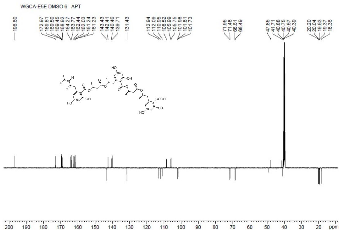
Figure S3-4. 13 C-NMR Spectrum of Compound 3
