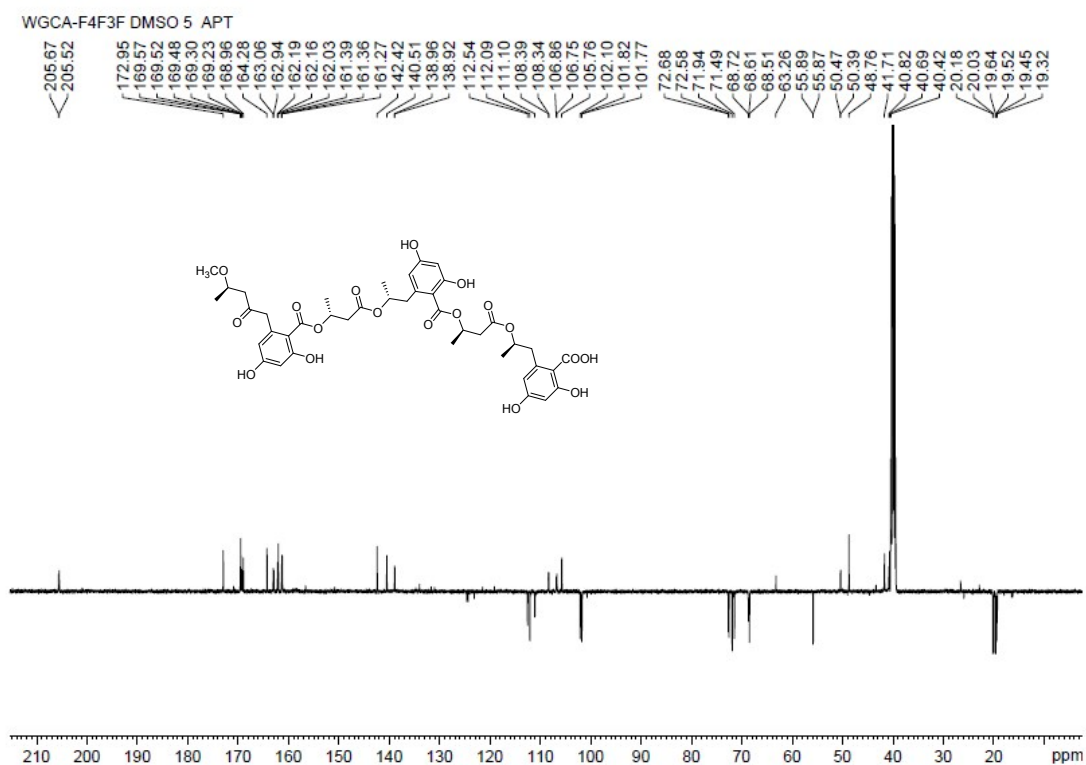
Figure S7-4. APT Spectrum of Compound 7
