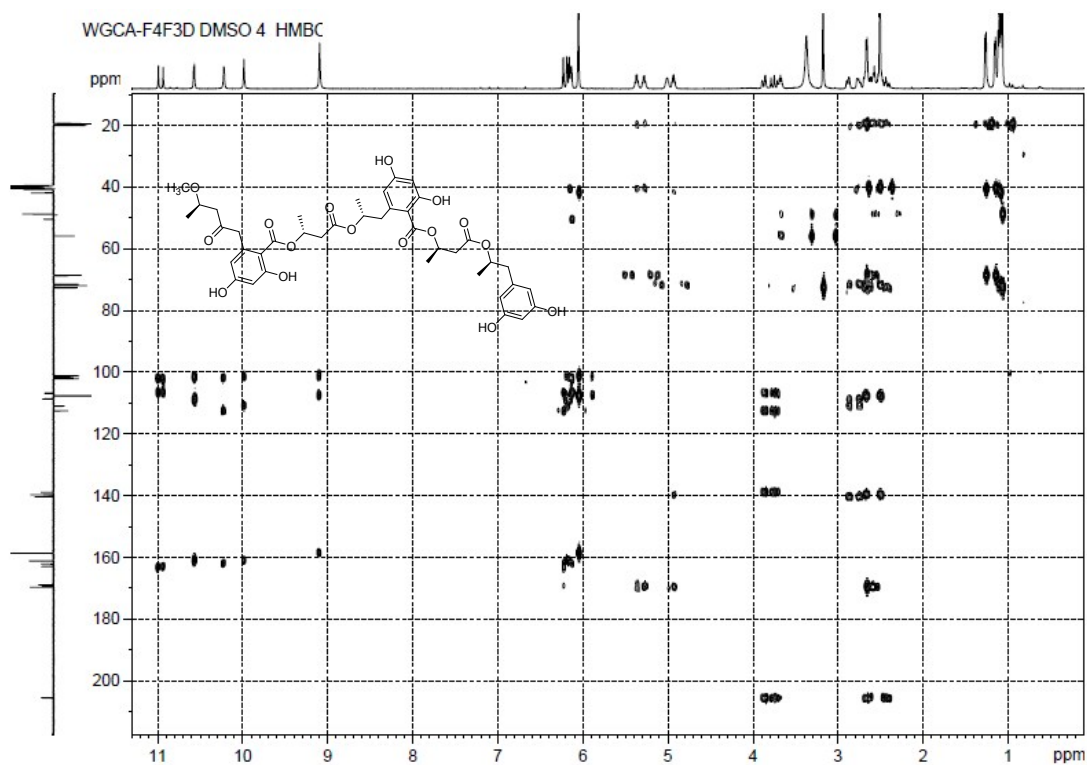
Figure S6-7. HMBC Spectrum of Compound 6
