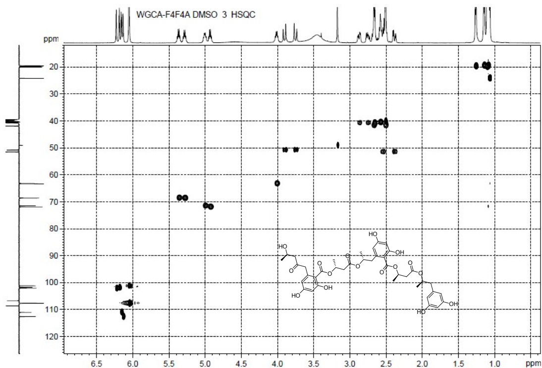
Figure S5-6. HSQC Spectrum of Compound 5
