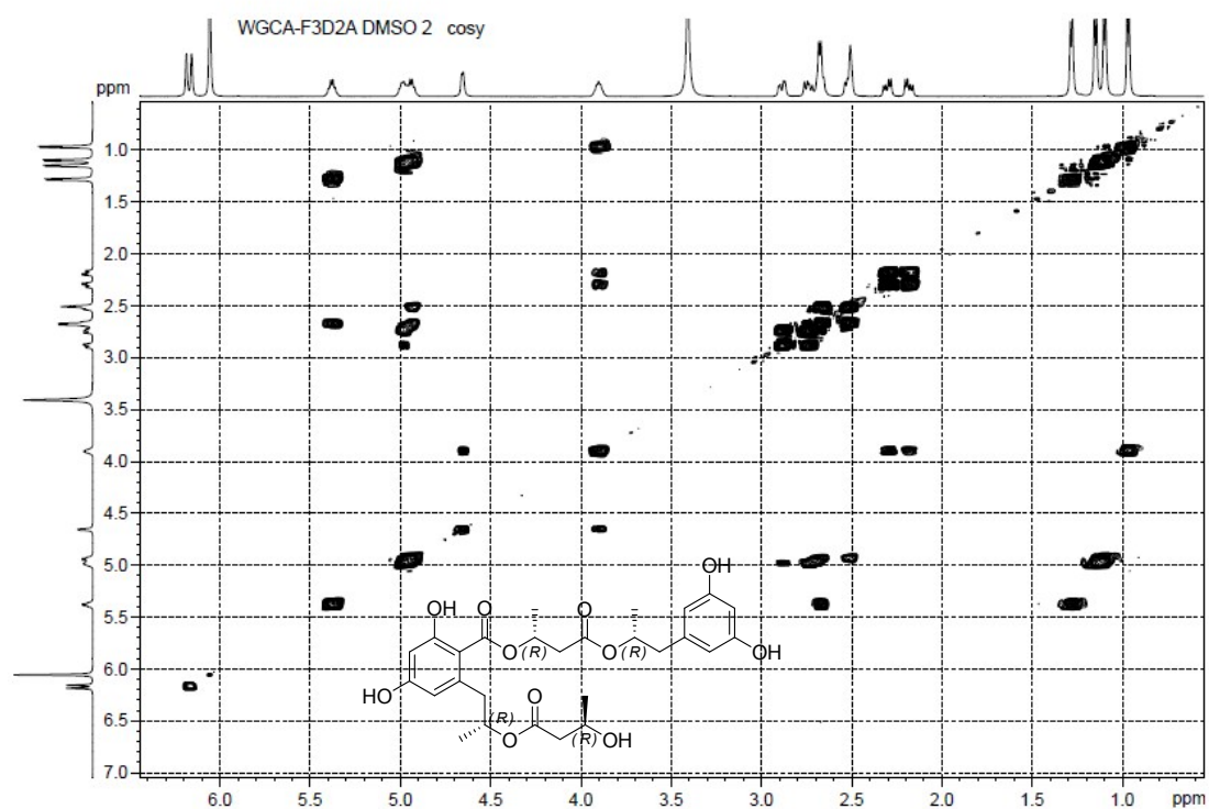
Figure S10-5. COSY Spectrum of Compound 10
