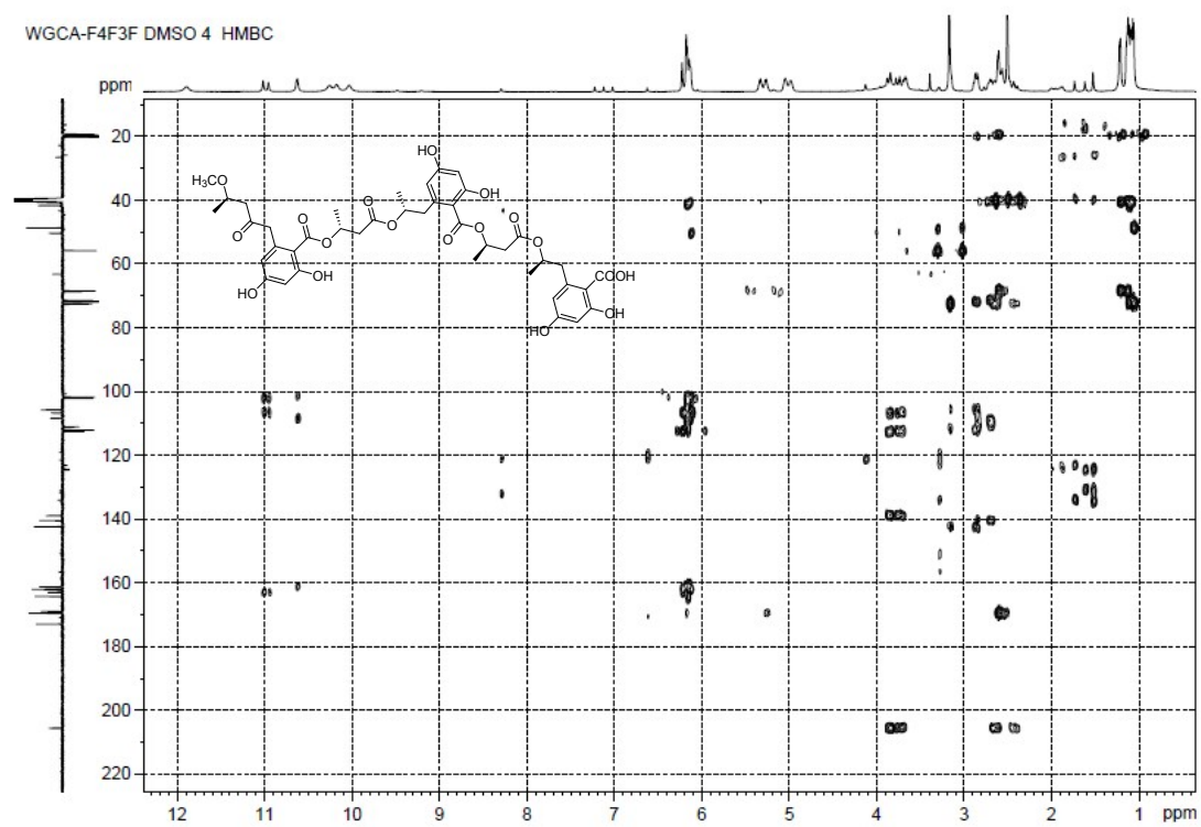
Figure S7-7. HMBC Spectrum of Compound 7
