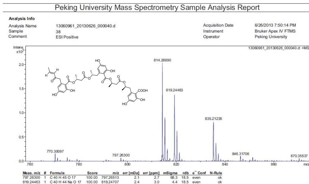
Figure S3-1. HRESIMS Spectrum of Compound 3
