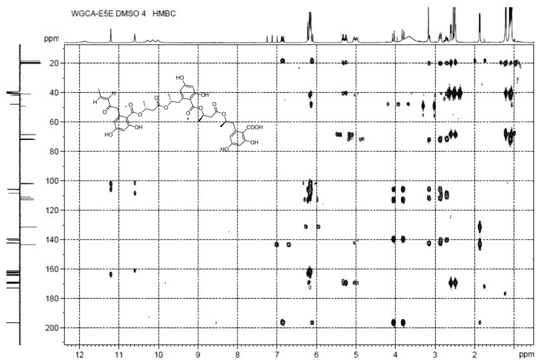
Figure S3-7. HMBC Spectrum of Compound 3
