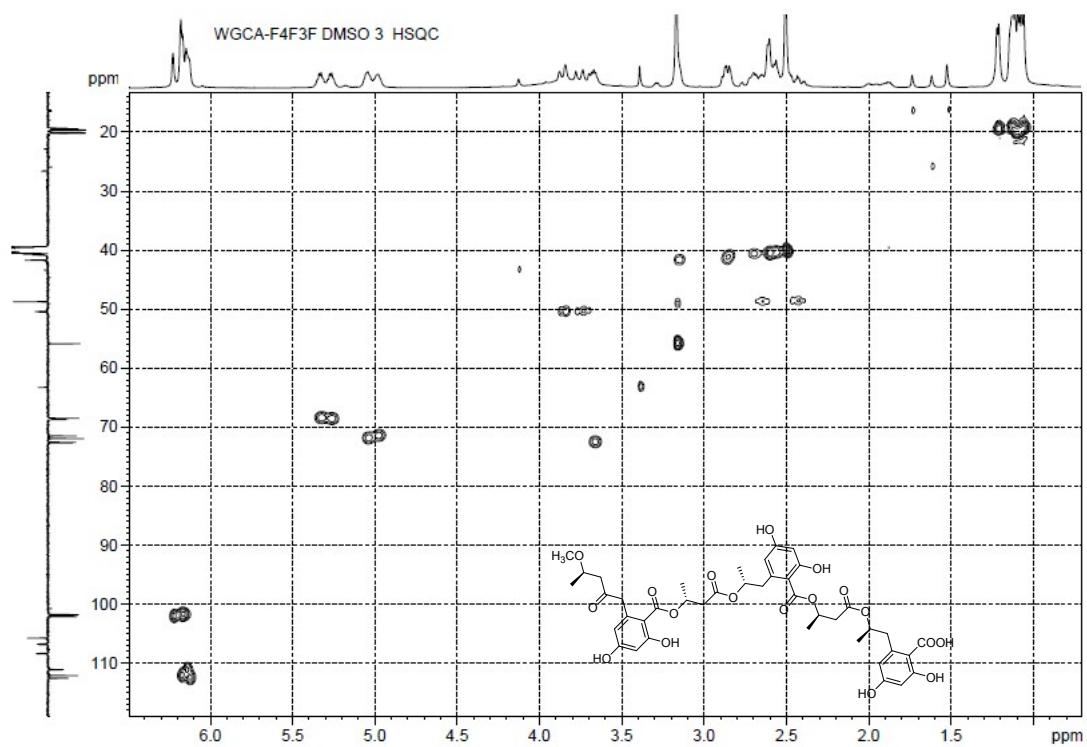
Figure S7-6. HSQC Spectrum of Compound 7
