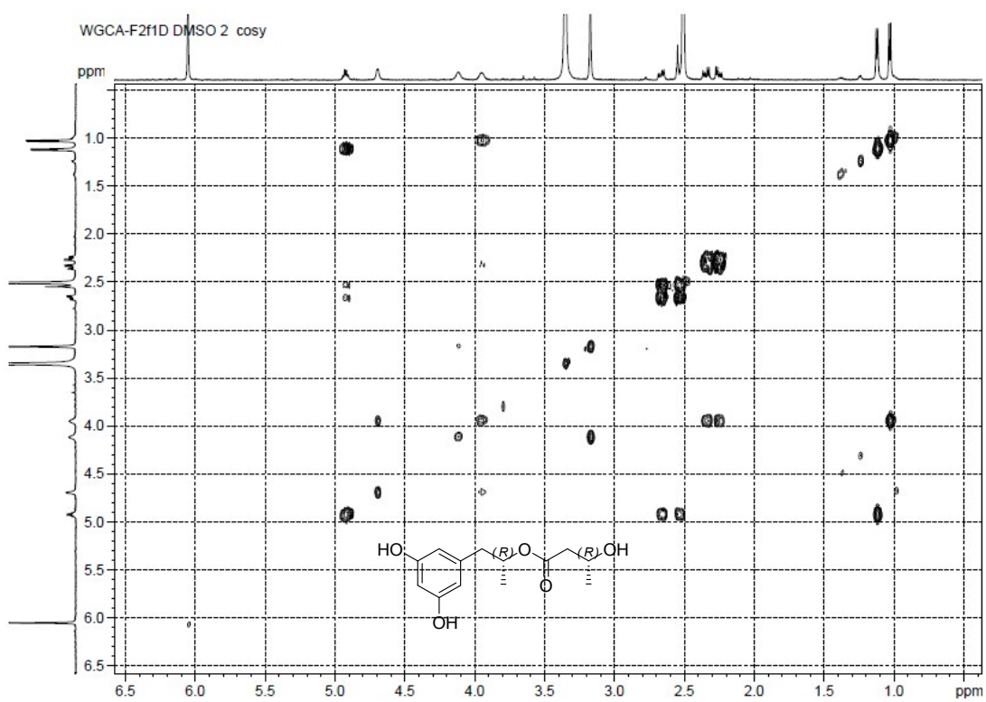
Figure S13-5. COSY Spectrum of Compound 13
