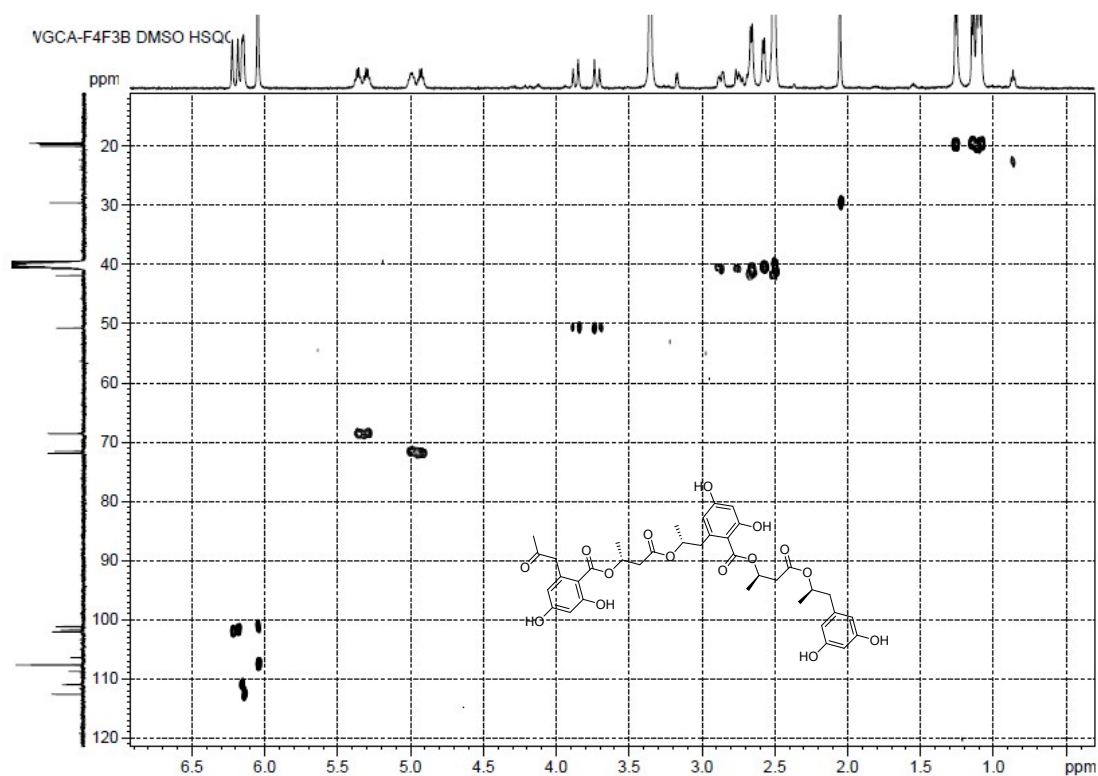
Figure S4-6. HSQC Spectrum of Compound 4
