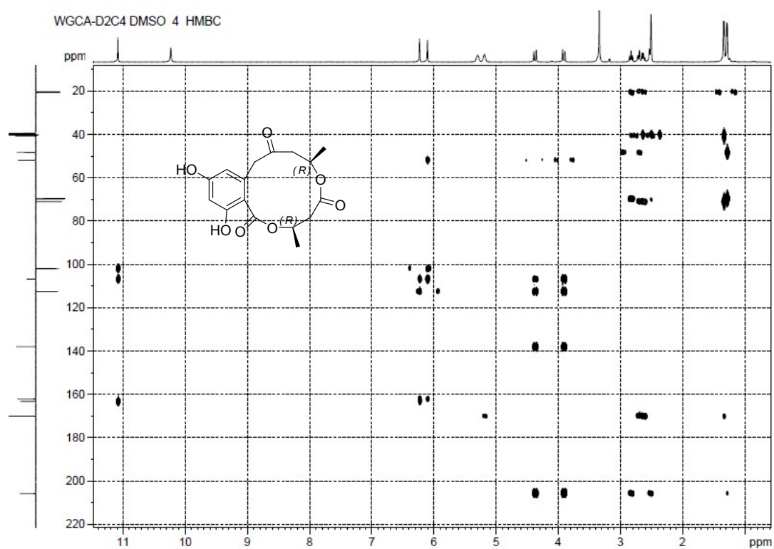
Figure S12-7. HMBC Spectrum of Compound 12
