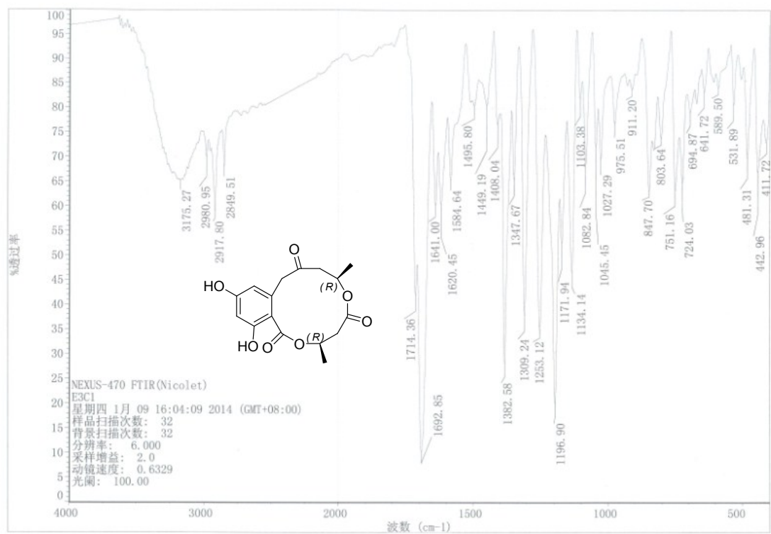
Figure S12-2. IR Spectrum of Compound 12
