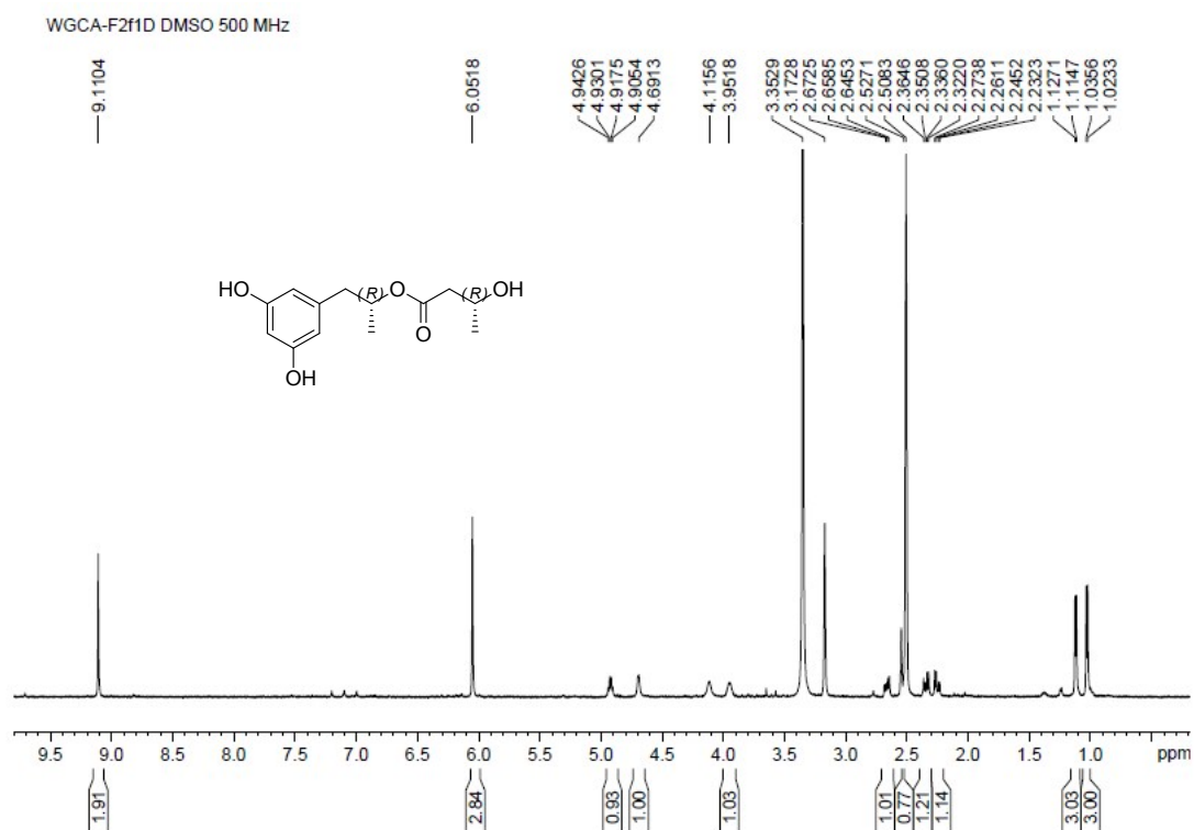
Figure S13-3. 1 H-NMR Spectrum of Compound 13
