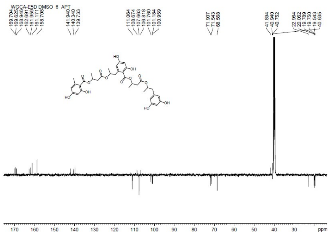
Figure S1-4. APT Spectrum of Compound 1
