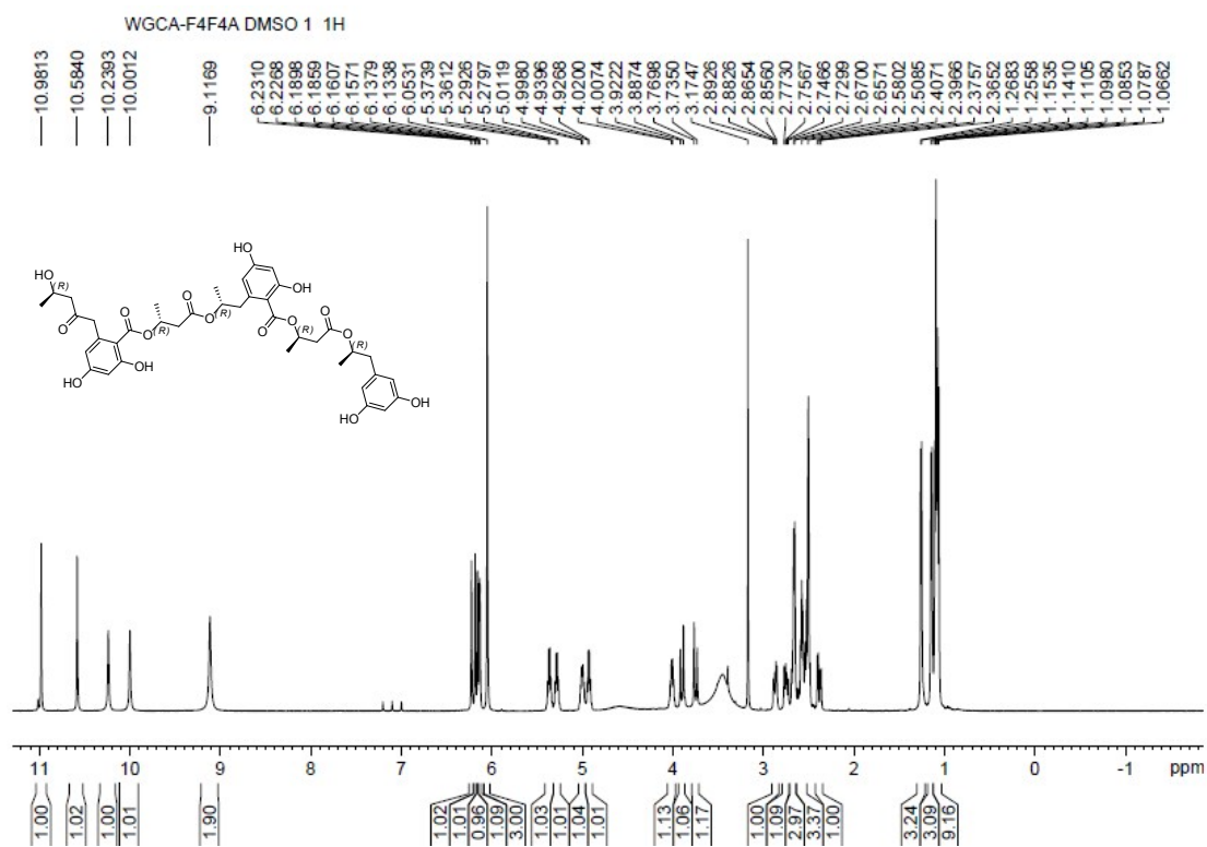
Figure S5-3. 1 H-NMR Spectrum of Compound 5
