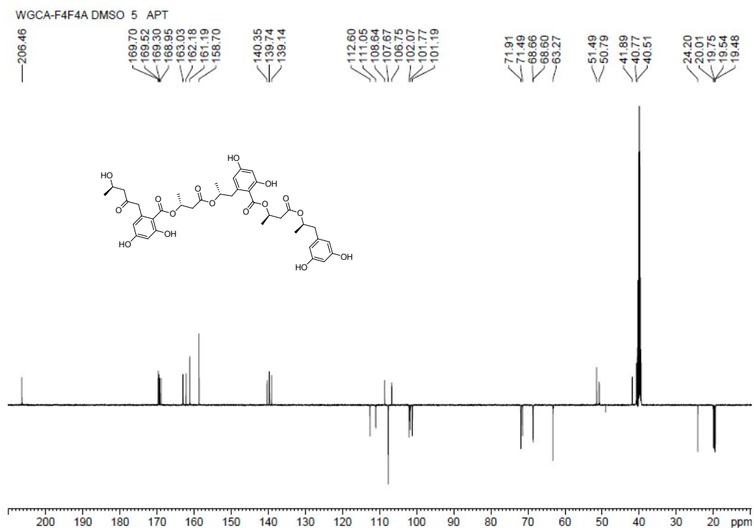
Figure S5-4. APT Spectrum of Compound 5
