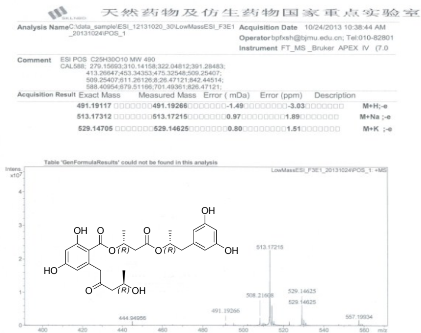
Figure S11-1. HRESIMS Spectrum of Compound 11
