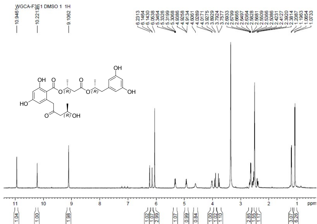
Figure S11-3. 1 H-NMR Spectrum of Compound 11
