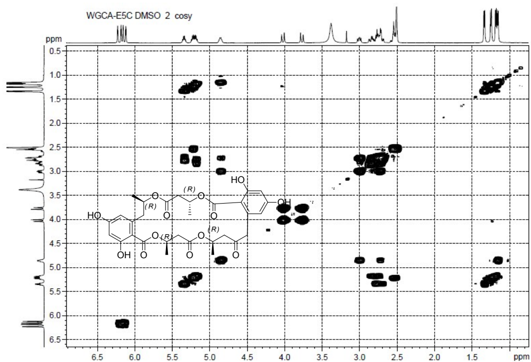
Figure S8-5. COSY Spectrum of Compound 8
