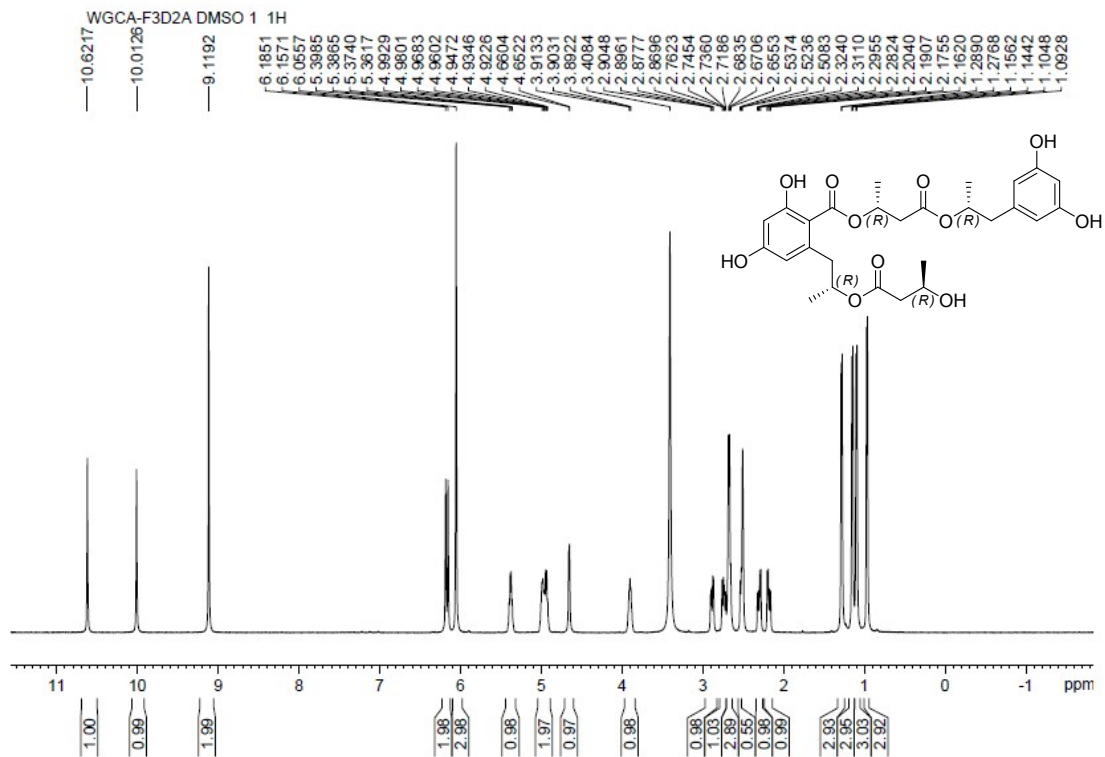
Figure S10-3. 1 H-NMR Spectrum of Compound 10
