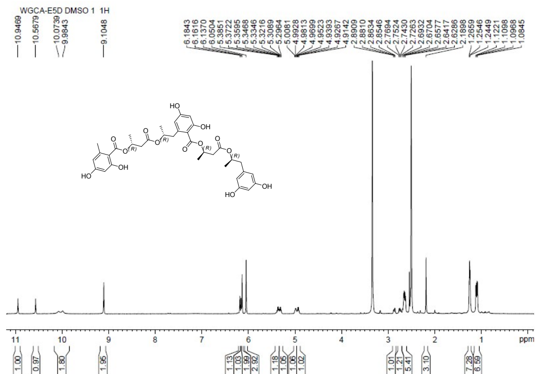
Figure S1-3. 1 H-NMR Spectrum of Compound 1
