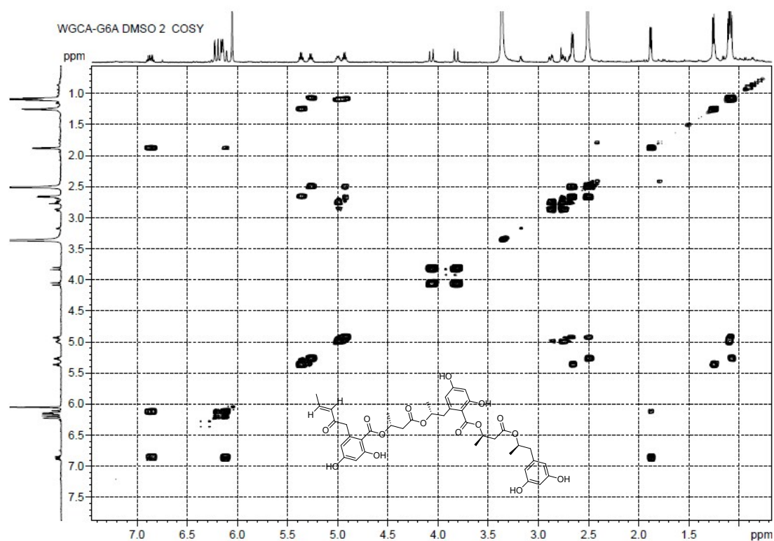
Figure S2-5. COSY Spectrum of Compound 2
