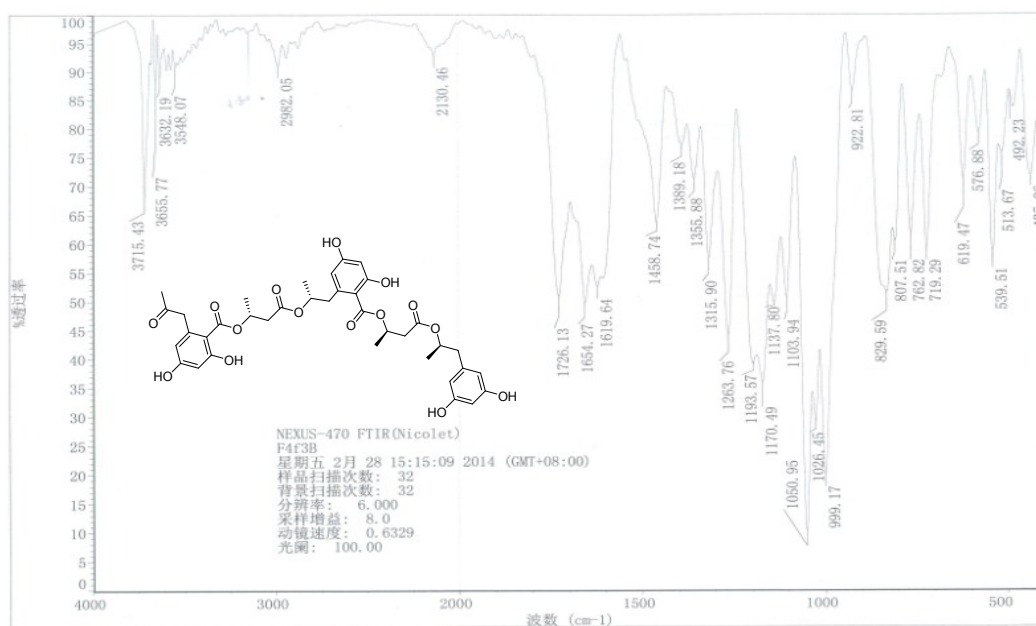
Figure S4-2. IR Spectrum of Compound 4
