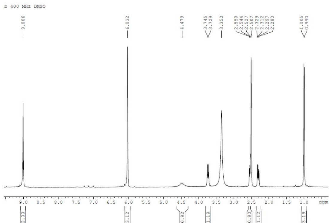
Figure Sb-1. 1 H-NMR Spectrum of 1d
