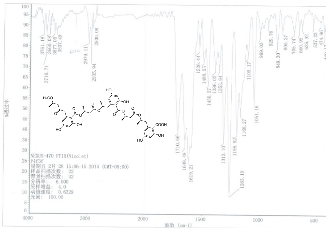
Figure S7-2. IR Spectrum of Compound 7
