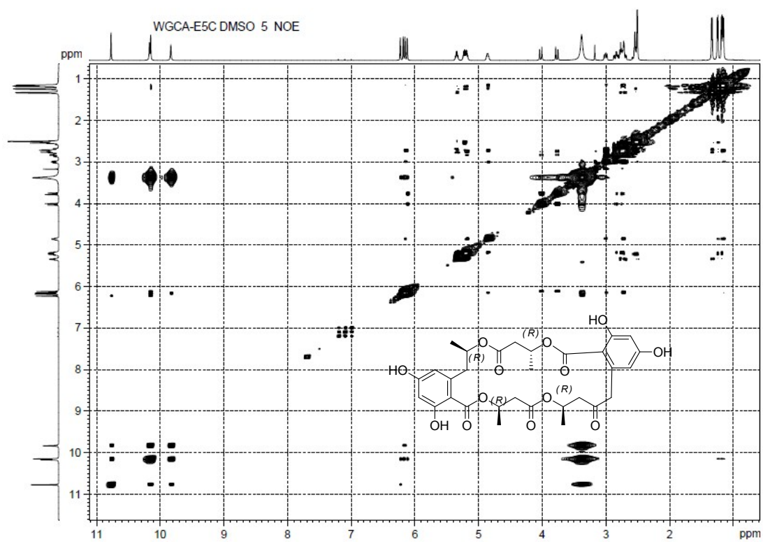
Figure S8-8. NOESY Spectrum of Compound 8
