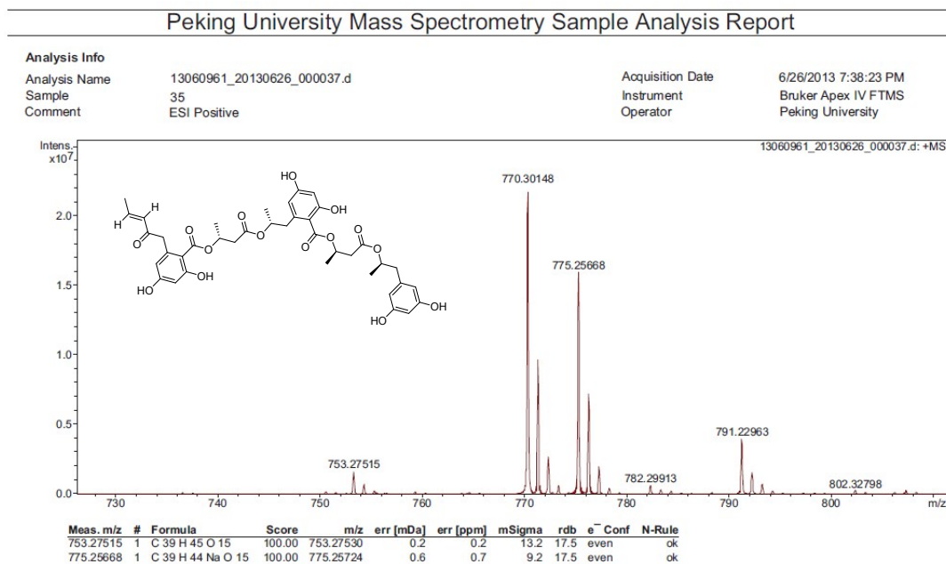
Figure S2-1. HRESIMS Spectrum of Compound 2
