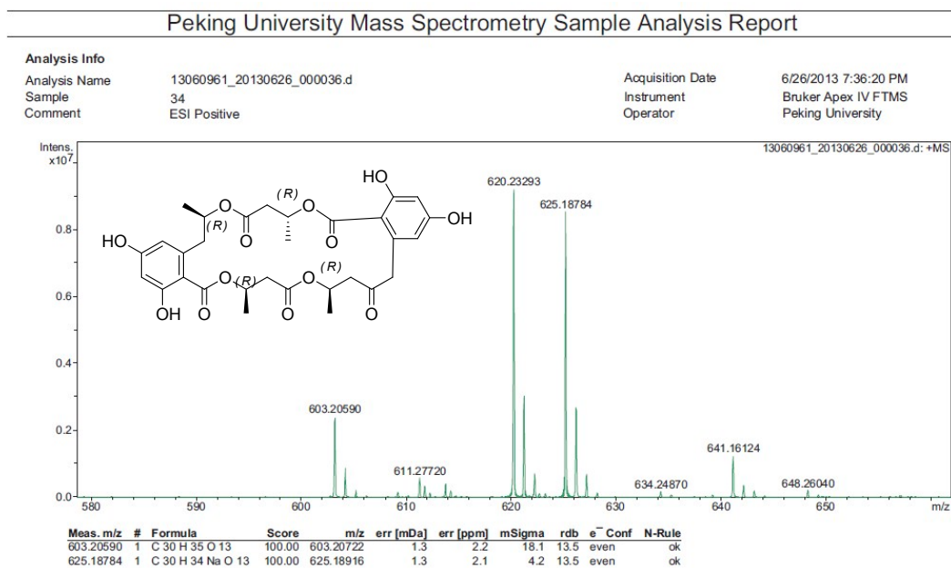
Figure S8-1. HRESIMS Spectrum of Compound 8
