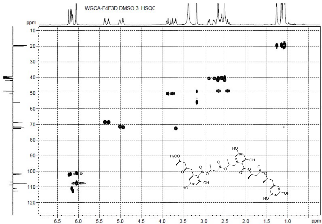
Figure S6-6. HSQC Spectrum of Compound 6
