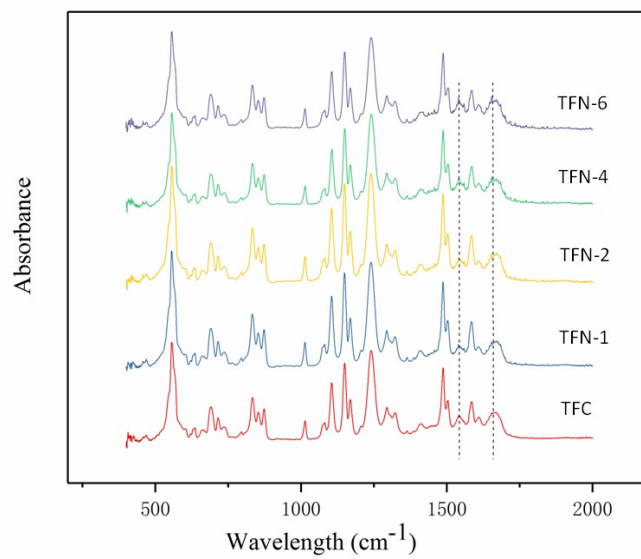
Fig. S2. FTIR spectra of TFC and TFN membranes
