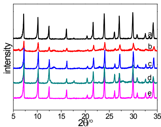
Fig. S1 Powder X-ray diffraction patterns for Ca-A and Ca-MA-x zeolites: a:Ca-A-0; b: Ca-MA-1; c: Ca-MA-2; d: Ca-MA-3; e: Ca-MA-4.
