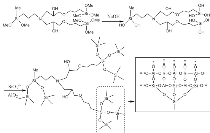
Scheme S1 Hydrolysis behavior and condensation mechanism of bridged polysilsesquioxane with silicate solution.
