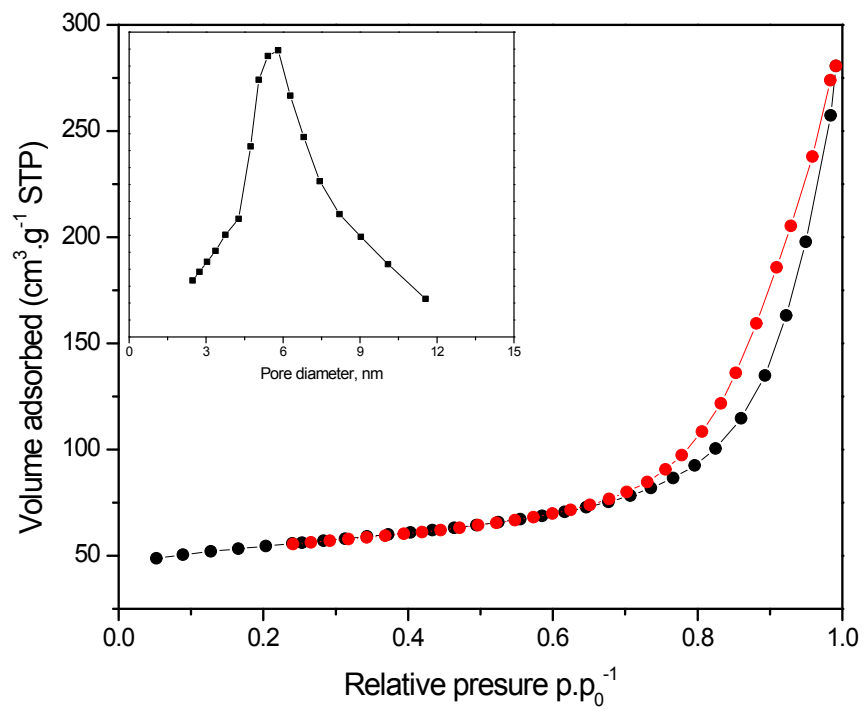
Figure S2. N 2 adsorption/desorption isotherms of mesoporous HSO 3 -ZSM-5 zeolite.
