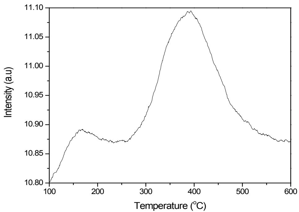
Figure S3. NH 3 -TPD profiles of the of mesoporous HSO 3 -ZSM-5 zeolite
