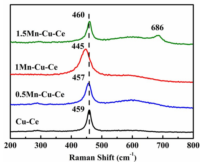
Fig. S1 Raman spectra of the as-synthesized catalysts.
