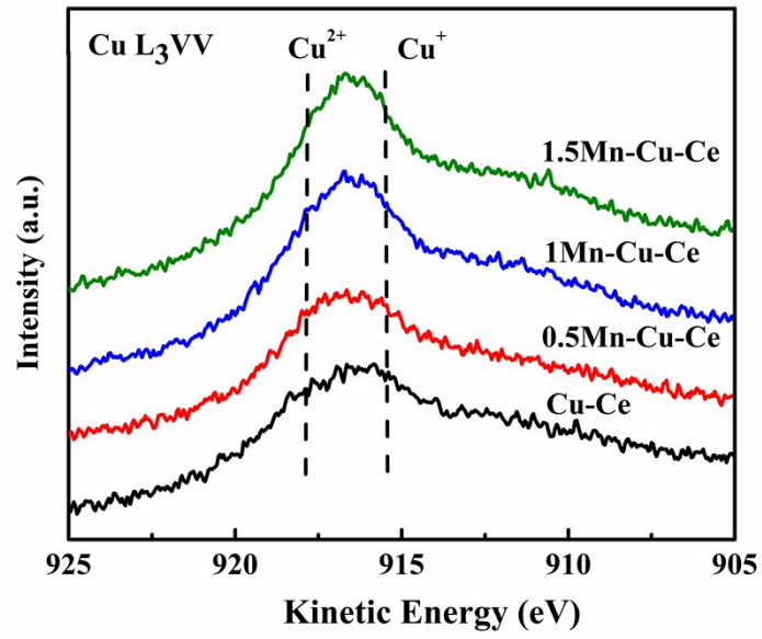
Fig. S2 Kinetic energy spectra of Cu L 3 VV Auger of the as-synthesized samples
