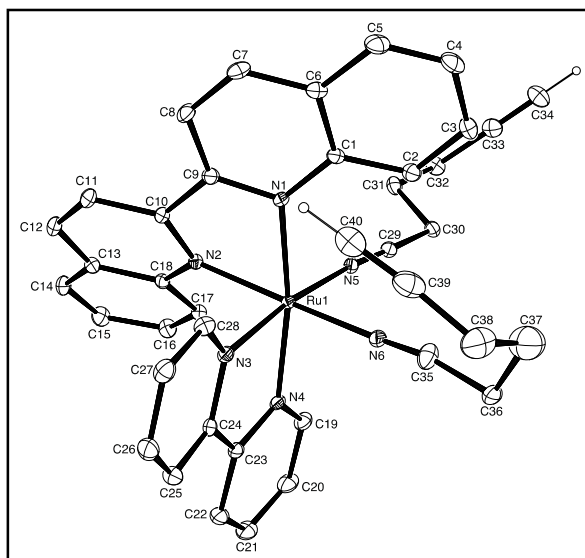
Figure S8 – Crystal Structure Determination of Ru(biq)(bpy)(5-hexynenitrile) 2 [PF 6 ] 2
