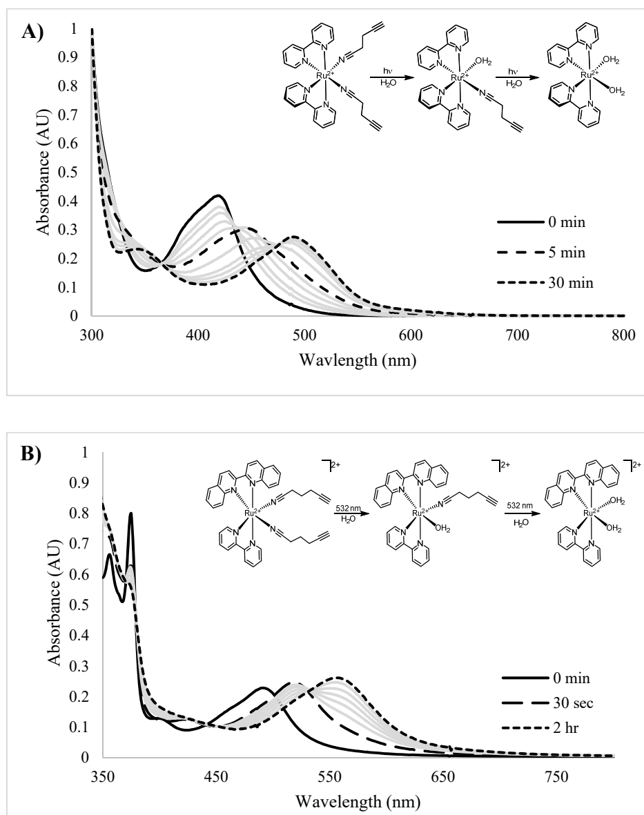
Figure S2 – Photolysis of 1 and 2
