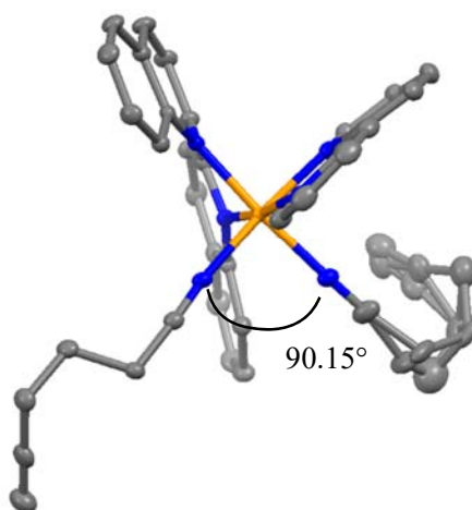
Figure S5. Crystal structure for 2 synthesized under longer, higher temperature reaction conditions. One 5-hexynenitrile ligand shows cis isomerization with 100% occupancy in the structure. The alkyne-biquinoline distance for the cis -hexyne was 3.734 Å, while the alkyne-biquinoline distance for the trans -hexyne was 6.809 Å. The cis product was observed after extended reaction times during the initial synthesis, and was irreversible.
