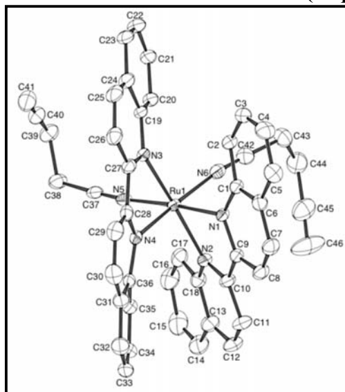
Figure S9 – Crystal Structure Determination of Ru(biq) 2 (4-pentynenitrile) 2
