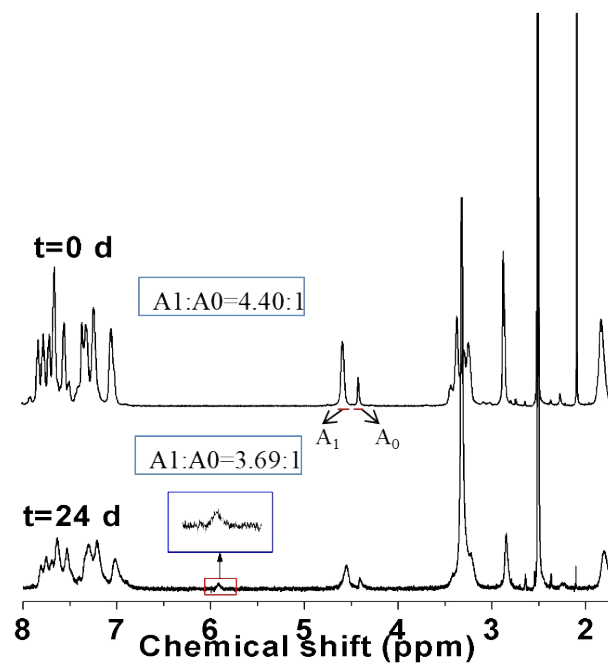
Fig S3. ^1\text{H} NMR spectrum of AEMs based from QPEEK-MPRD in OH- form before and after storage in 1 M NaOH at 60 °C for 24 days.
