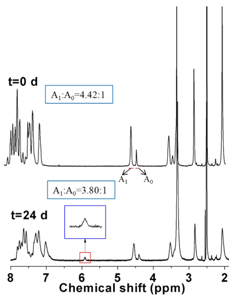
Fig S2. 1 H NMR spectrum of AEMs based from QPEEK-MPY in OH- form before and after storage in 1 M NaOH at 60 °C for 24 days.
