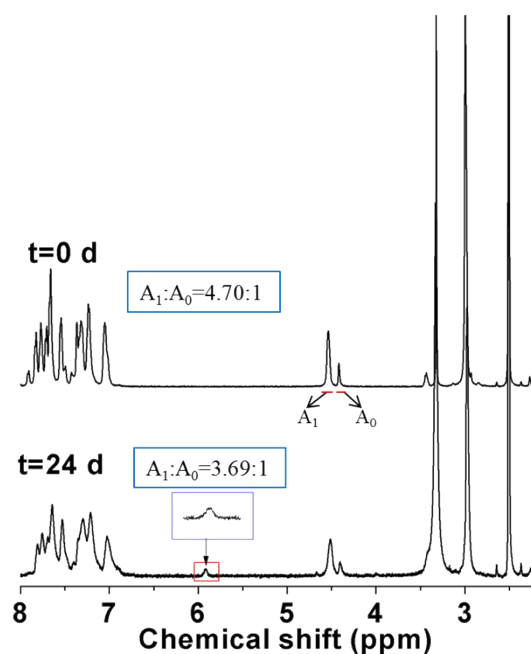
Fig S1. 1 H NMR spectrum of AEMs based from QPEEK-TMA in OH- form before and after storage in 1 M NaOH at 60 °C for 24 days.
