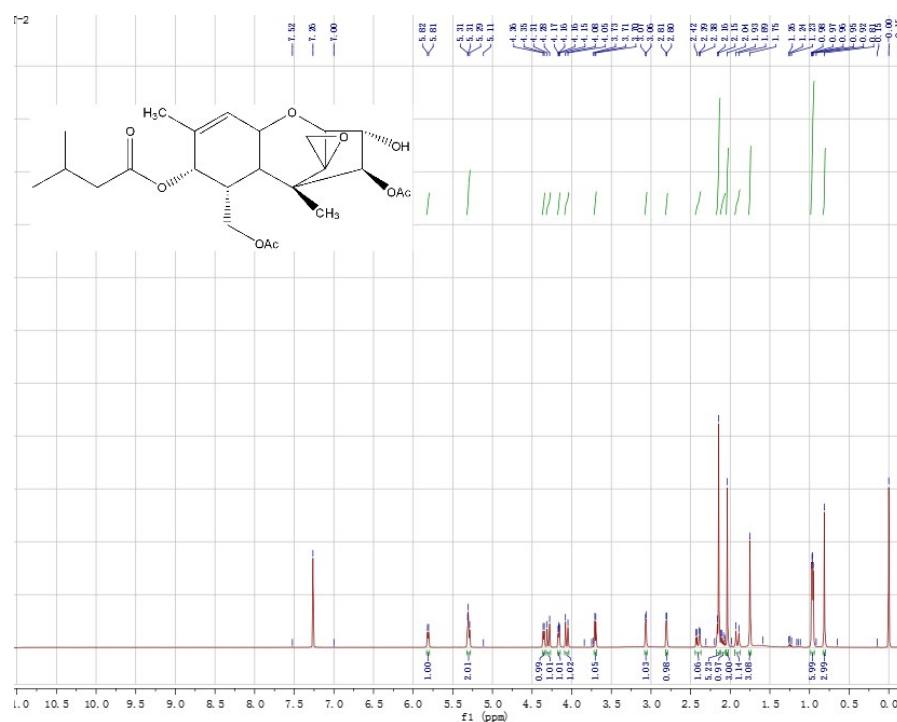
Fig S1. The NMR spectra (D 2 O, 600 MHz) of the T-2 toxin.
