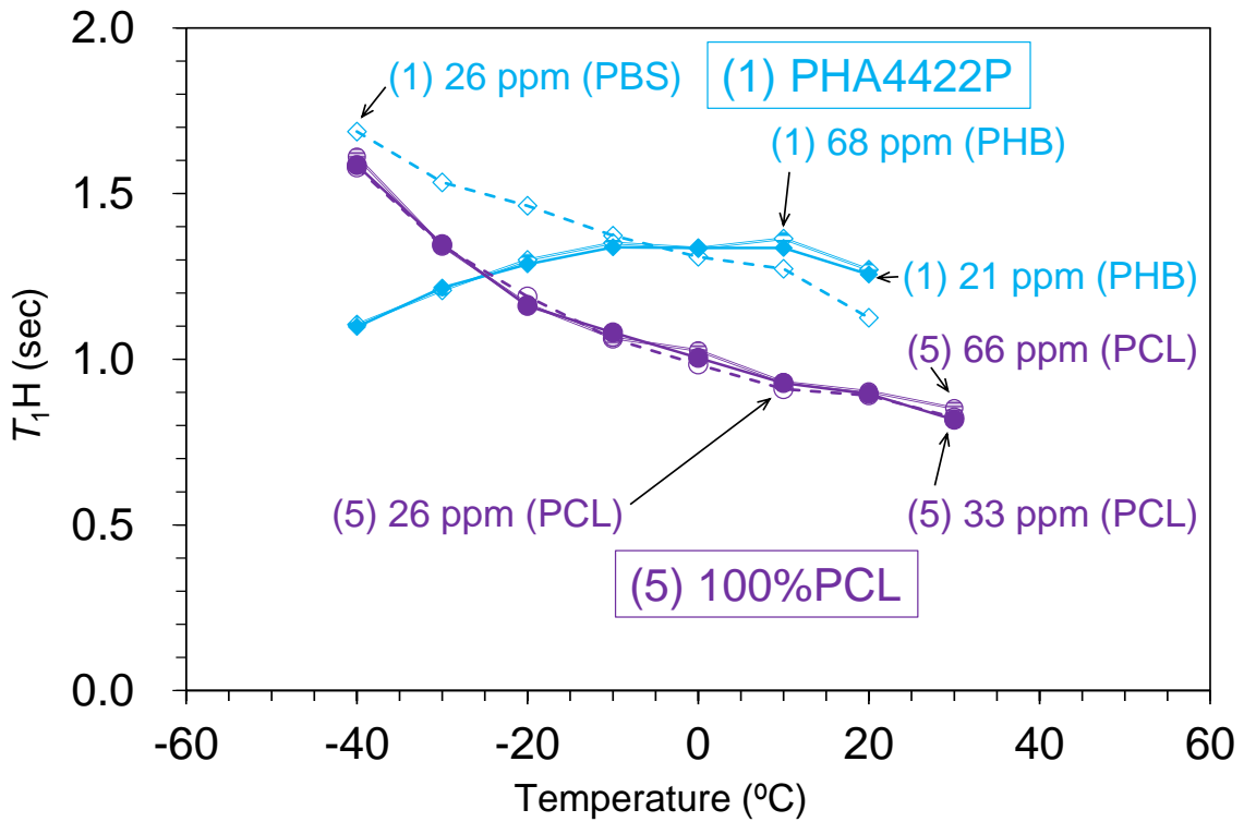
Fig. S2. T_{1H} changes of plasticized PHA (1) and PCL (5) with rising temperature.
