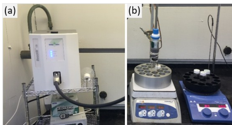
Fig. S1 Experimental set-up for 20 mL vial batch reaction kinetics study: (a) ReactIR 15, and (b) heating block for batch reaction
