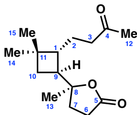
(+)-rumphellaone A (8)
