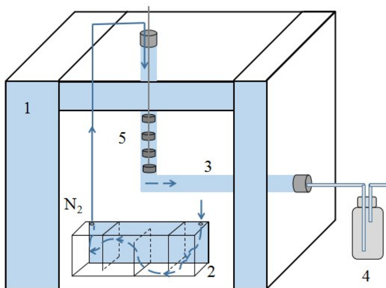
Supplement Fig. 1 The schematic of self-designed pyrolysis tubular reactor; (1) High temperature oven; (2) Gas preheating device; (3) Quartz tube; (4) Condensed product collection unit; (5) Quartz basket
