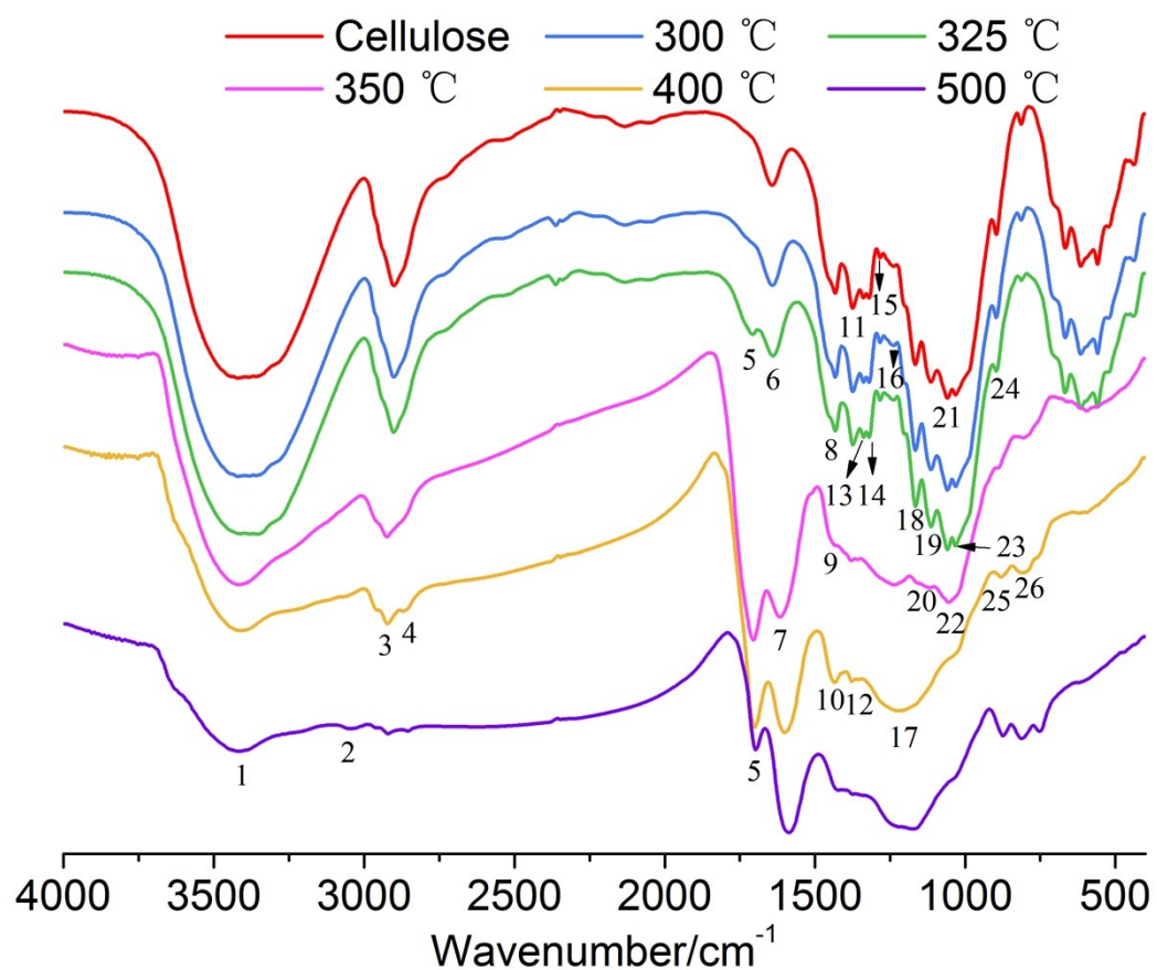
Supplement Fig. 3 FTIR spectra evolution of the cellulose slow pyrolysis process
