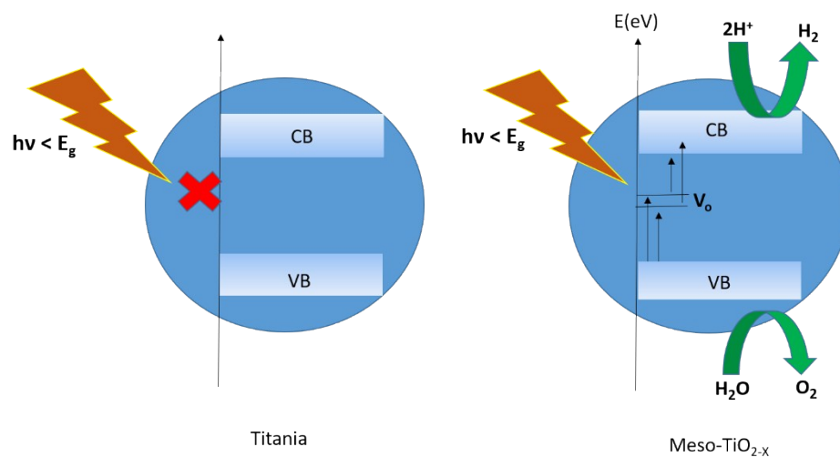
Figure S3. A schematic diagram showing lower energy visible light photon absorption by meso-TiO 2-x materials available in AM1.5 irradiation for photocatalysis.
