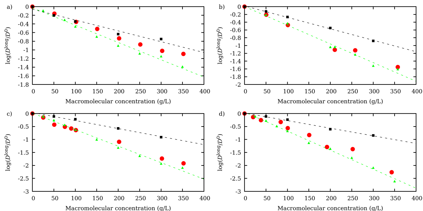
Fig. 1 \log(D^{\text{long}}/D_0) for streptavidin versus macromolecular concentration for D10 (a), D50 (b), D400 (c) and D700 (d). Black squares represent BD simulations using hard-sphere model as explained in 2 and green triangles correspond to BD simulations using CESP model. Experimental values 2 are depicted as red circles. Dashed lines follow the simulation results and they are only to guide the eyes.
