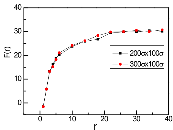
Figure. S1 Effective force F(r) between two anti-parallel wedges as a function of r at a particle density of \rho = 0.05 with the apex angle of \theta = 90^\circ for systems of 200\sigma \times 100\sigma and 300\sigma \times 100\sigma , respectively.
