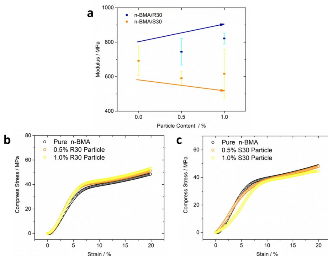
Figure S1. Compression measurements of PnBMA nanocomposites. (a) Compression modulus of PnBMA nanocomposite with two types of particles. (b, c) Compress stress-strain curves of PnBMA containing raspberry-like (b) and strawberry-like (c) particles with different weight percentages.
