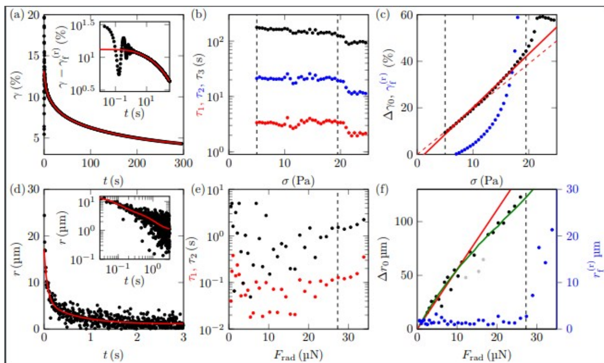
suppfig2_recovery_exponential
