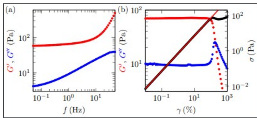
Suppfig1_oscillations
