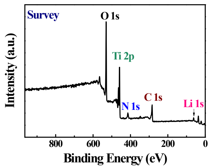
Figure S1. XPS survey spectrum of LTO/N-C nanotube arrays
