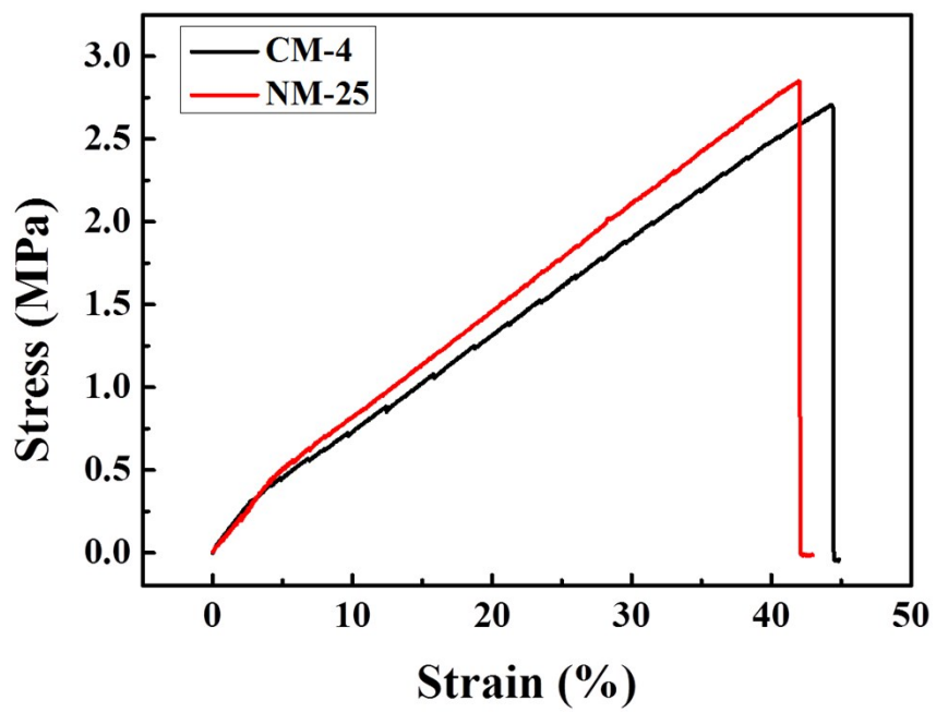
Figure S1. Stress-strain curves of NM-25 and CM-4 membrane.
