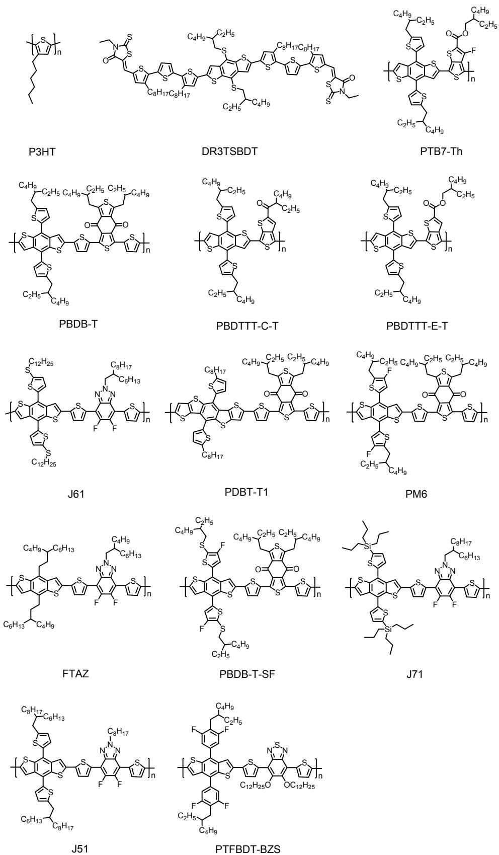
Fig. S1 Chemical structures of donors mentioned in the text.
