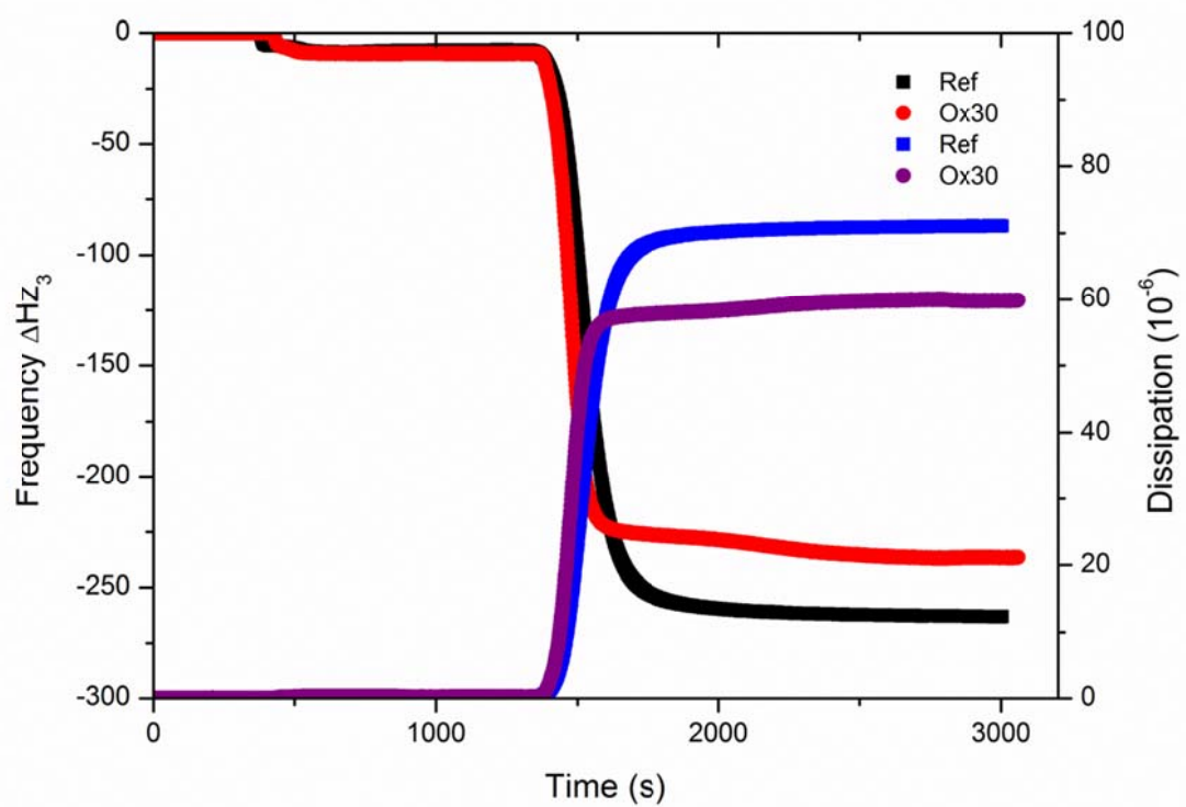
Figure 3. QCM-D data of frequency and dissipation change for the 3 rd overtone during adsorption of non-oxidized CNFs and Ox30 CNFs.
